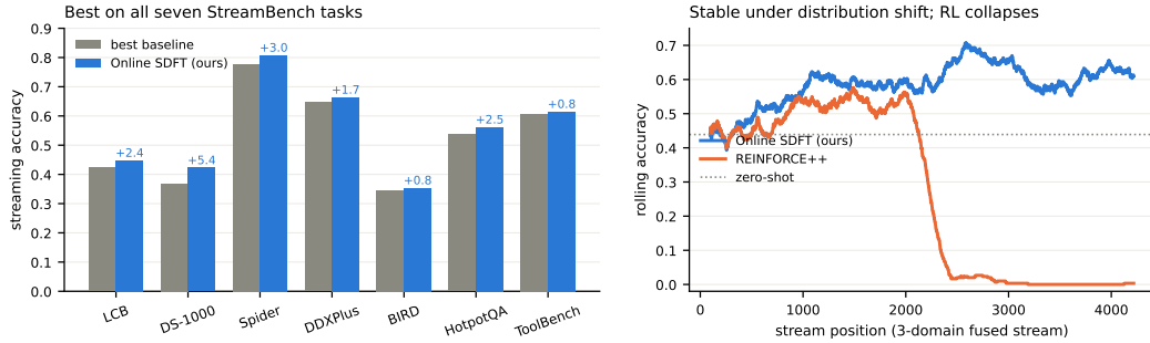
Figure 1: Left: final streaming accuracy on seven StreamBench tasks; Online SDFT (blue) exceeds the strongest baseline (zero-shot, Self-StreamICL, or REINFORCE++, gray) on every task. Right: rolling accuracy on a 4,219-problem stream interleaving three domains; Online SDFT improves throughout while REINFORCE++ collapses after roughly 2,000 problems.
