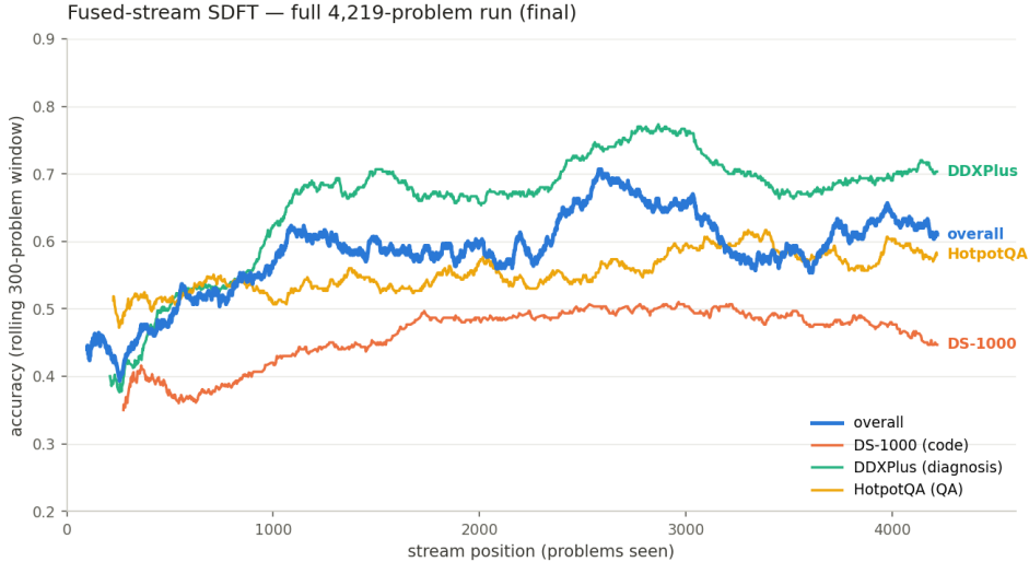
Figure 2: Rolling accuracy (300-problem window) of Online SDFT over the fused three-domain stream, overall and per domain. All domains improve simultaneously; no interference from distribution shift.
