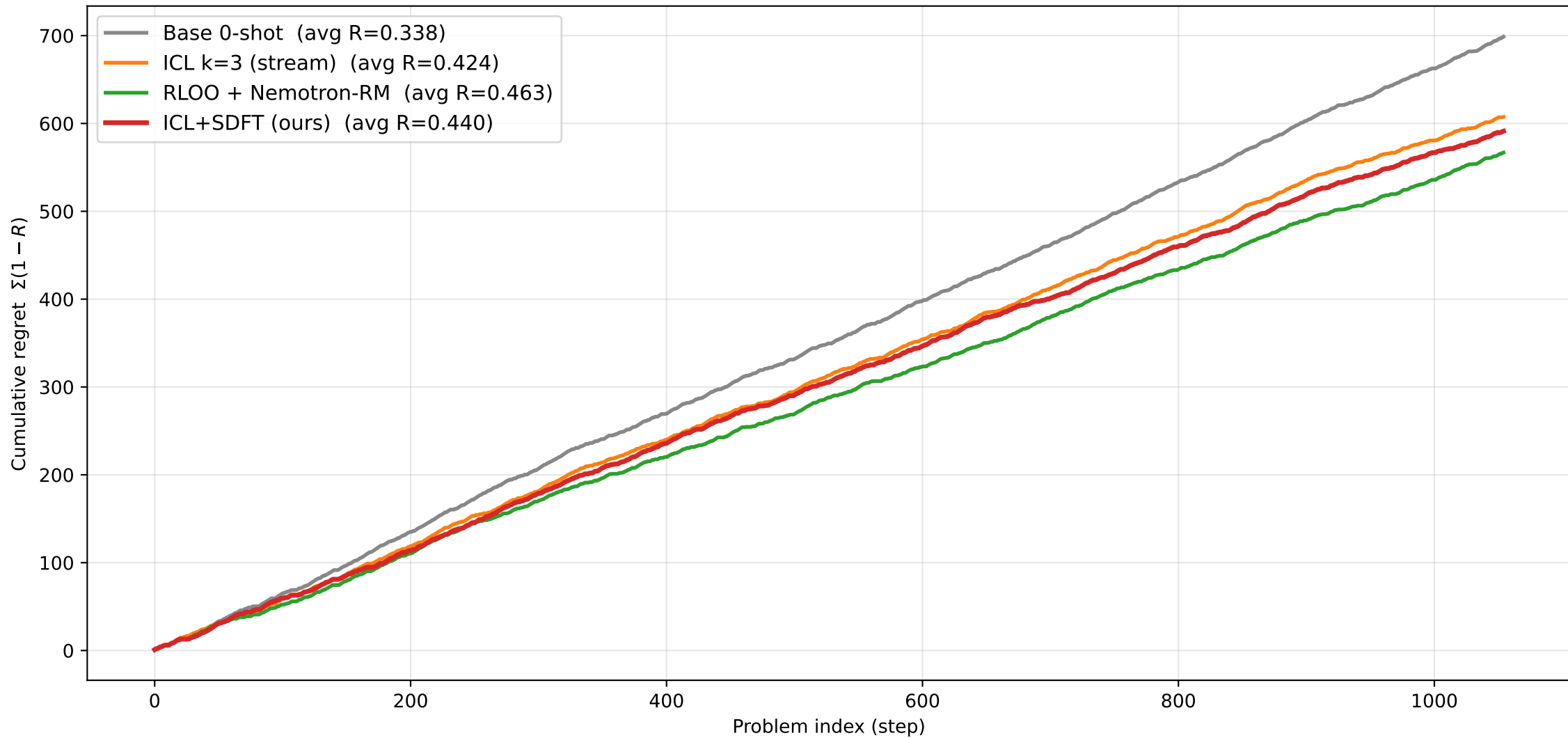
Online cumreg on LCB (1055 problems, Qwen2.5-Coder-7B, 1 oracle/q for eval)
