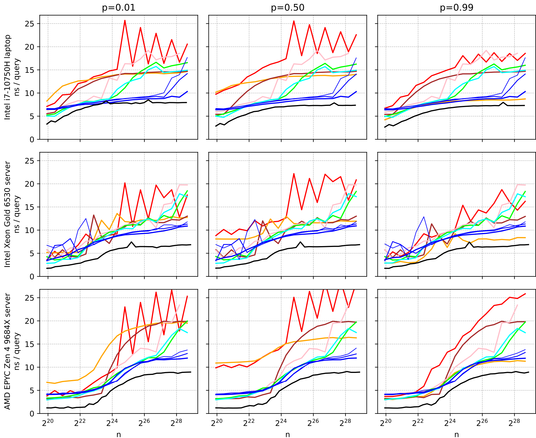
StaticHashset&lt;u64&gt; query throughput (1 thread, loop with prefetch)
