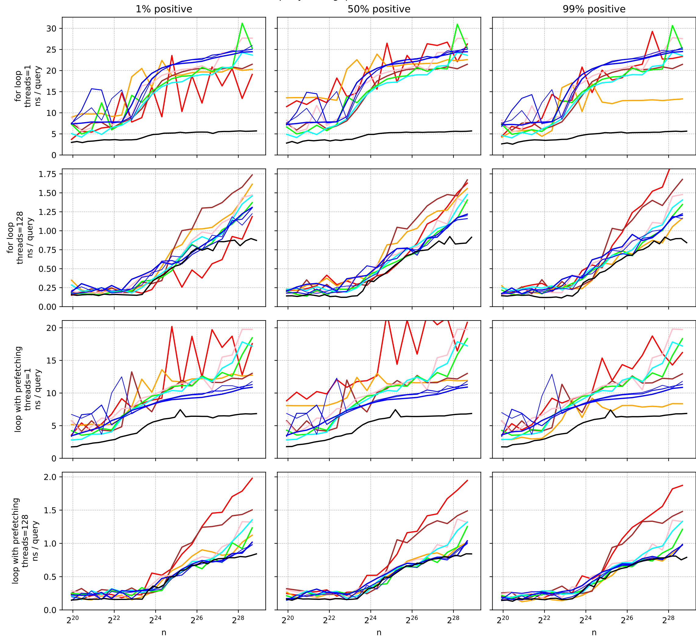
Hashset&lt;u64&gt; query throughput (Intel Xeon Gold 6530 server)
