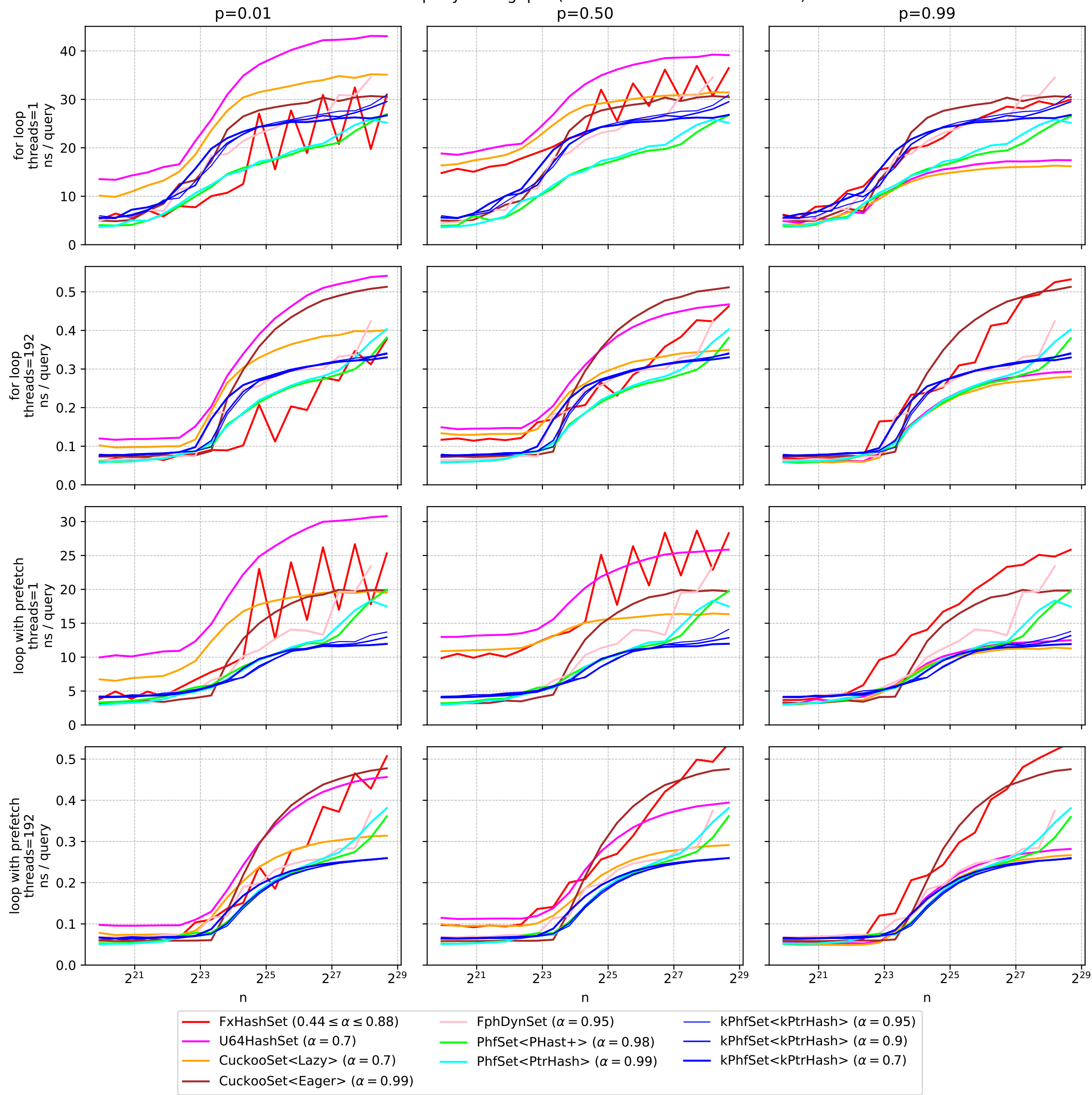
Hashset&lt;u64&gt; query throughput (AMD EPYC Zen 4 9684X server)
