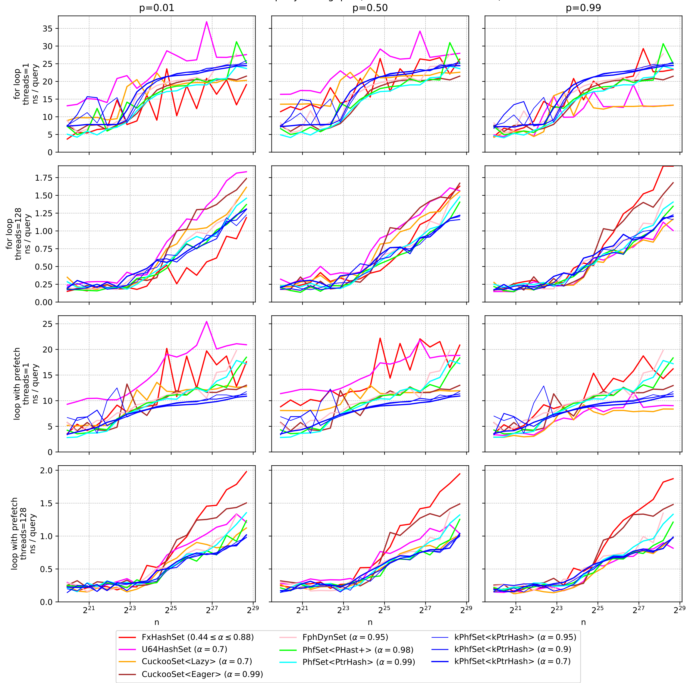
Hashset&lt;u64&gt; query throughput (Intel Xeon Gold 6530 server)
