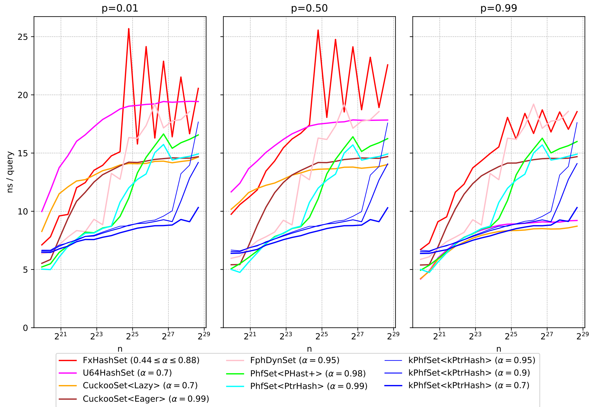
StaticHashSet<u64> query throughput (Intel i7-10750H laptop, 1 thread, loop with prefetch)
