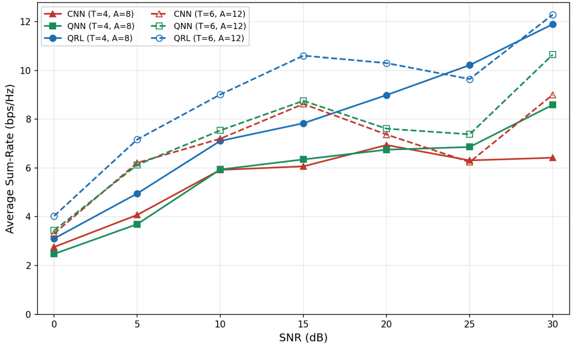
Fig. 6 — Sum-rate vs SNR for QNN, CNN, and QRL under different user-antenna configurations
