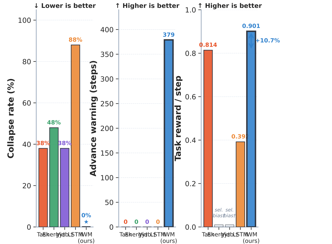
(C) The Result (FeverAnt, 5 seeds, 50 episodes)
