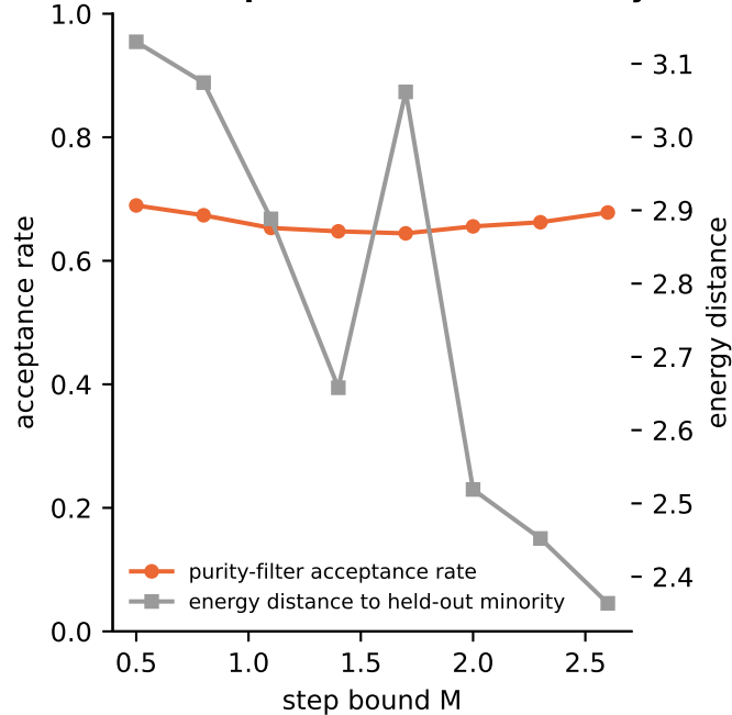
B. Acceptance and admissibility vs M
