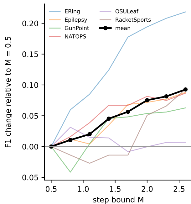
C. Downstream F1 vs M (IR = 10)
