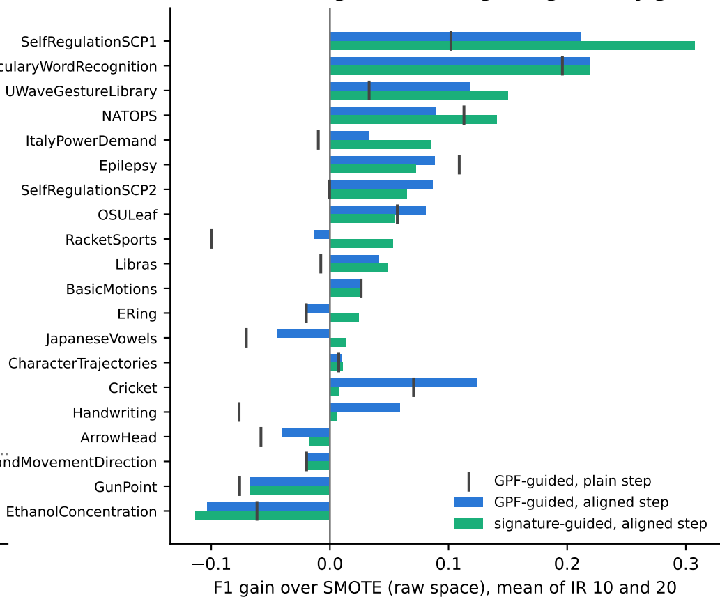
B. Per-dataset gain of the aligned, geometry-guided walk
