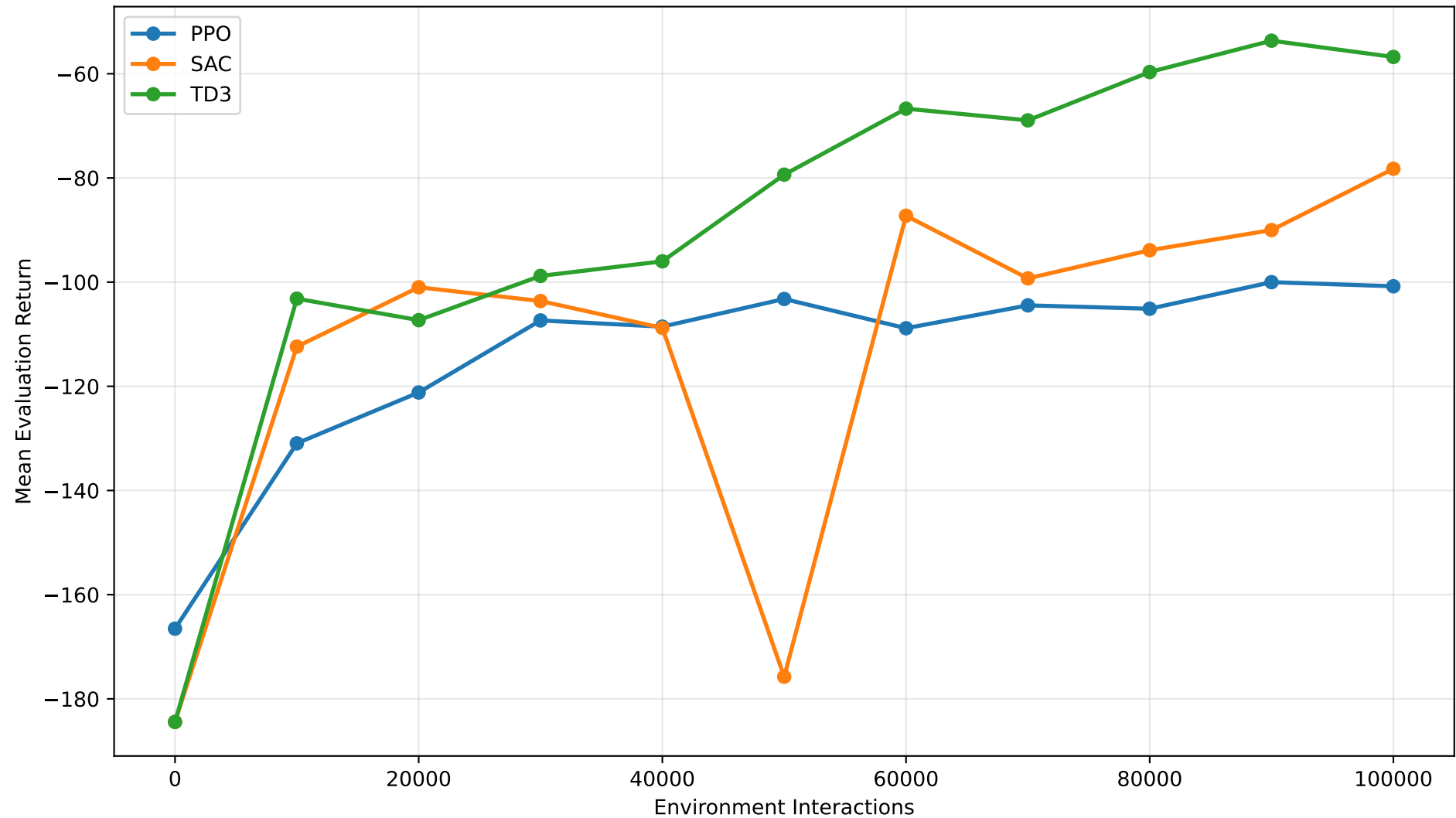
Mean Evaluation Return During Training
