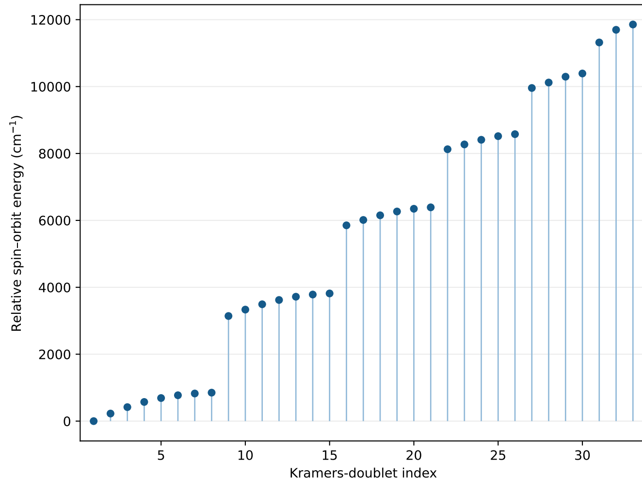
All 33 Kramers doublets
