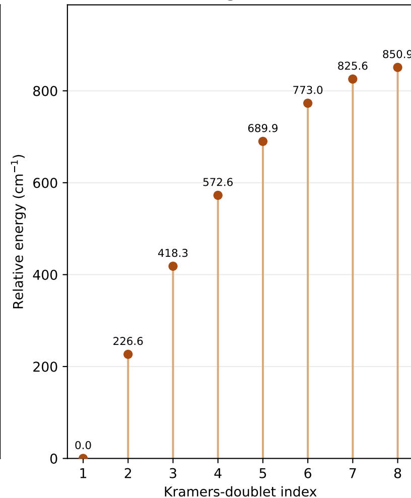
Lowest eight doublets
