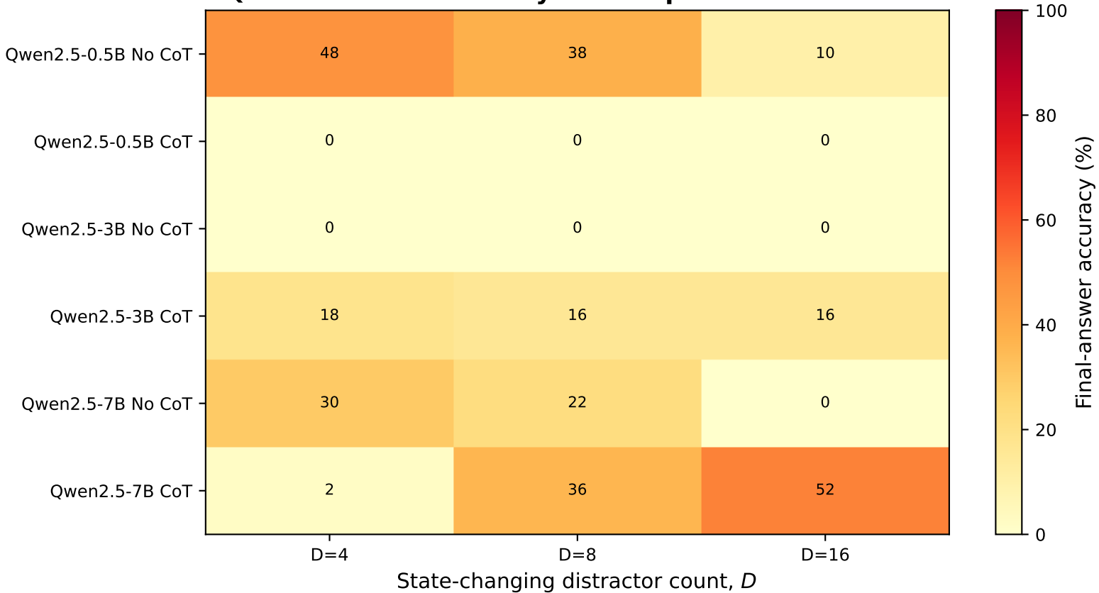
RQ3: Distractor accuracy heatmap
