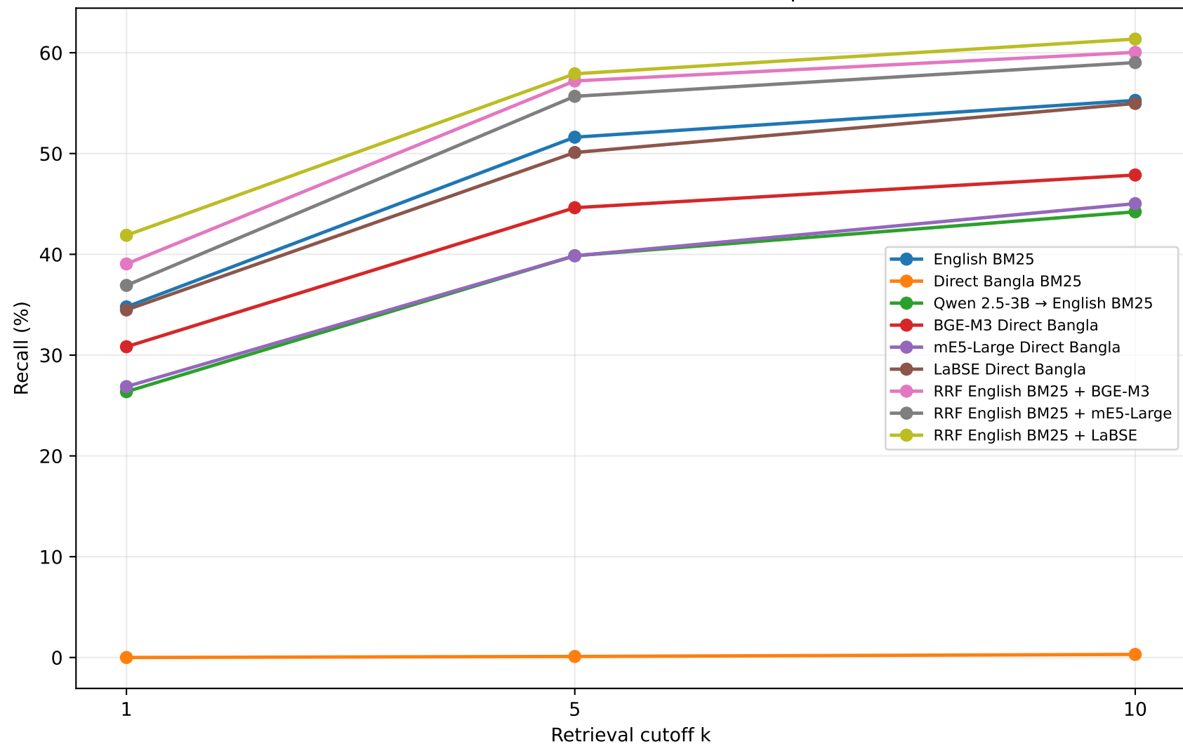
Recall Growth with Retrieval Depth
