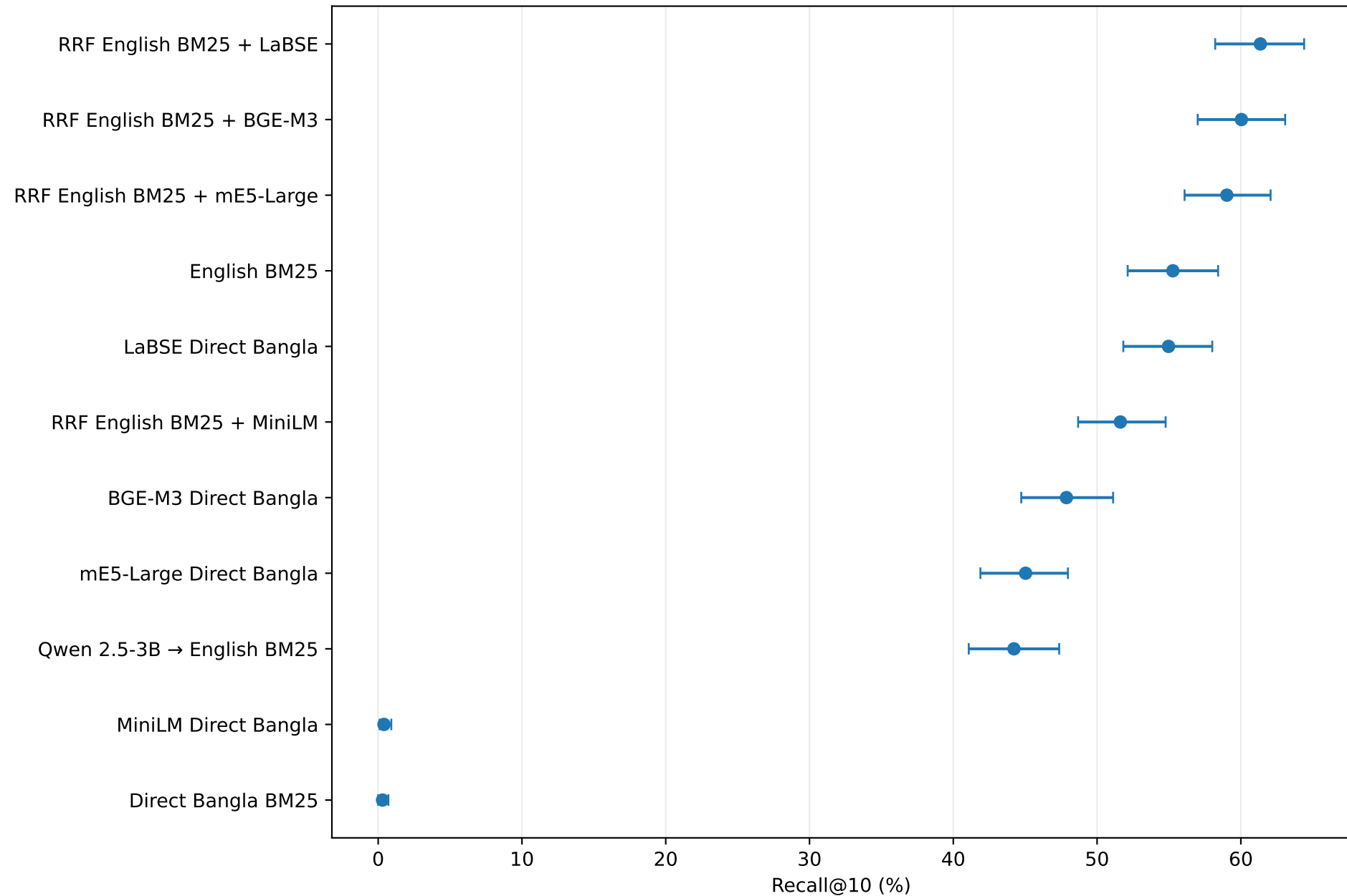
Recall@10 with 95% Bootstrap Confidence Intervals
