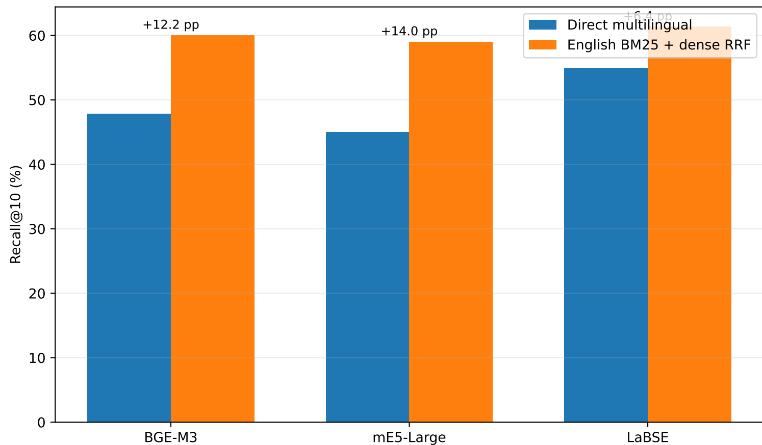
Effect of Lexical-Semantic Rank Fusion
