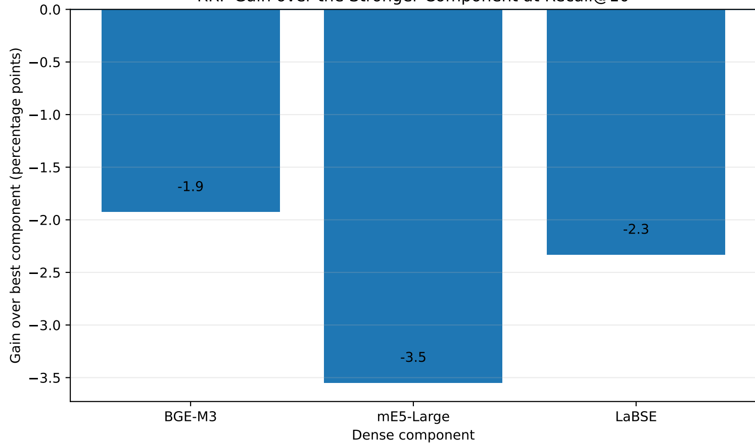
RRF Gain over the Stronger Component at Recall@10
