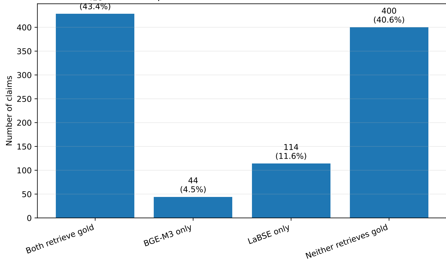
Paired Top-10 Retrieval Outcomes: BGE-M3 vs. LaBSE
