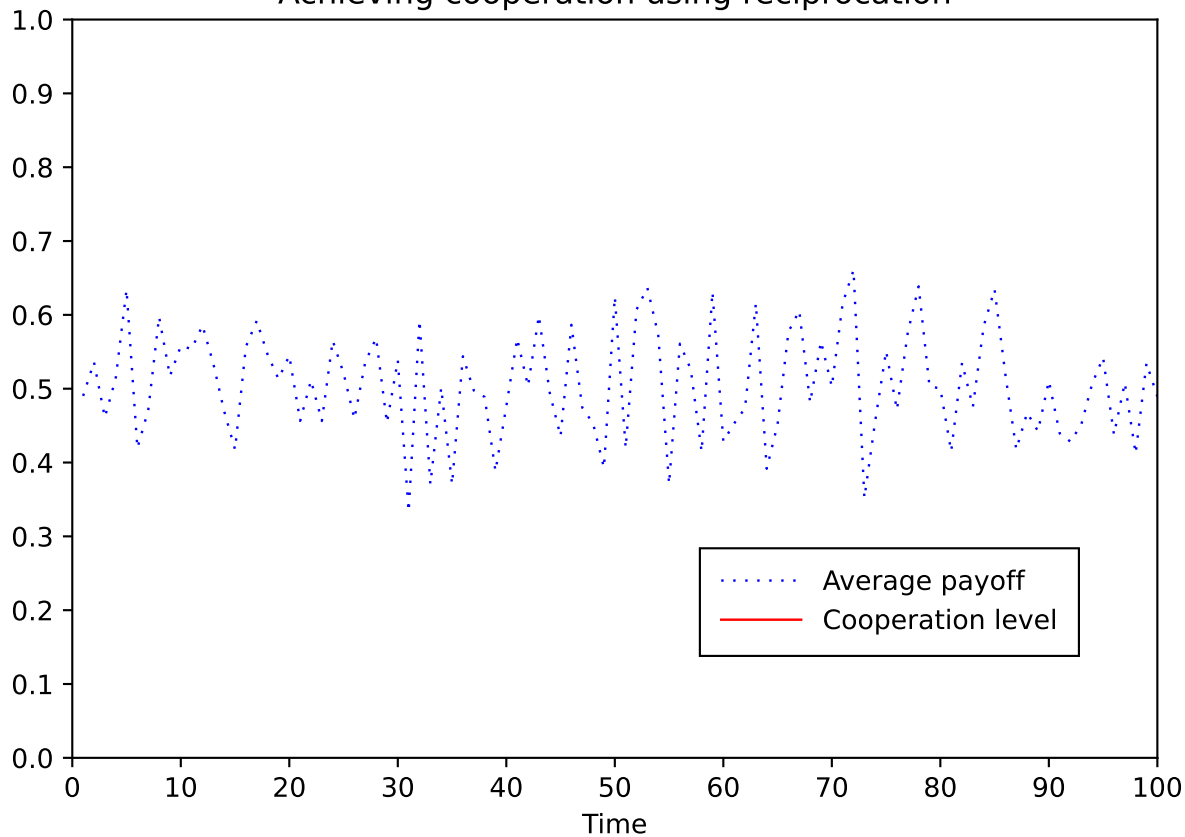
Achieving cooperation using reciprocity
