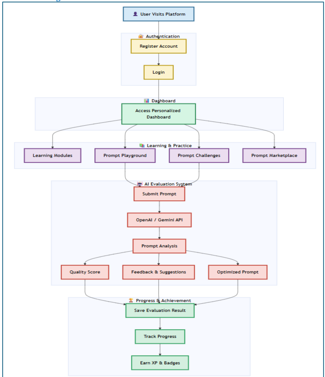
Figure 19: User Flow Diagram
