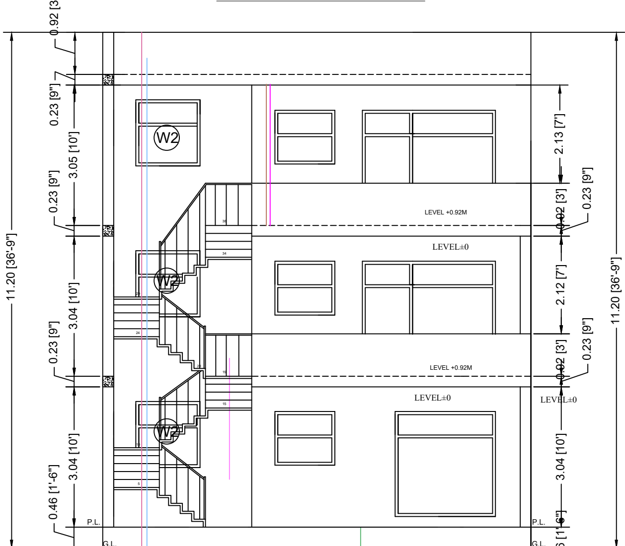
FRONT ELEVATION
