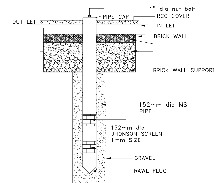
SECTION RAIN WATER HARVESTING PIT
