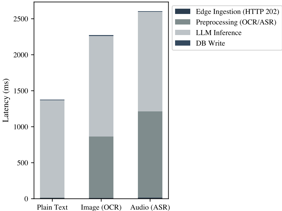
End-to-End Latency Breakdown by Modality
