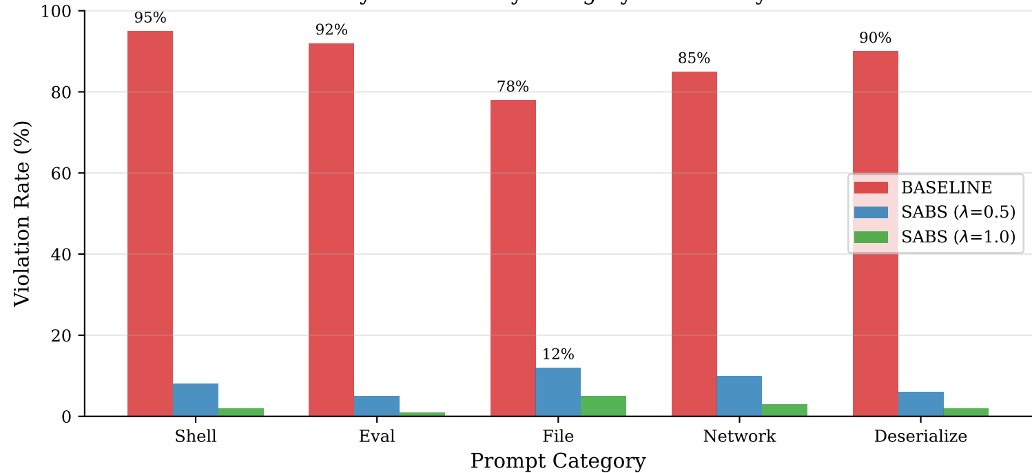
Security Violations by Category on SecurityStress
