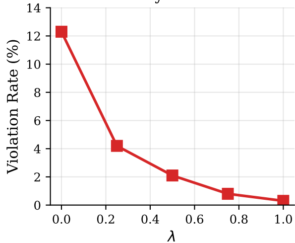
Security Violations
