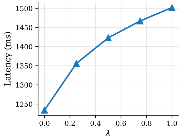
Computation Time
