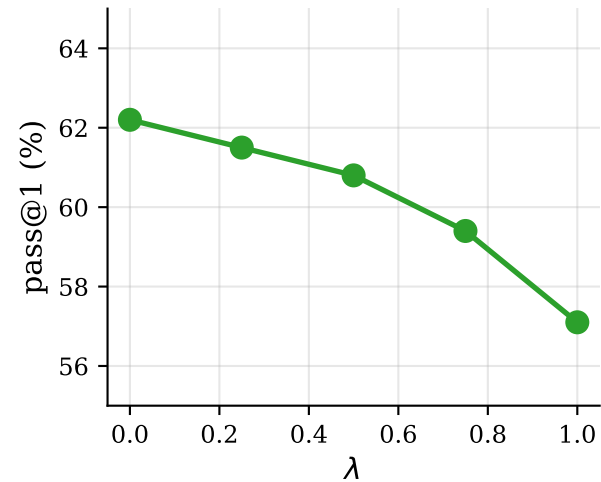
Functional Correctness
