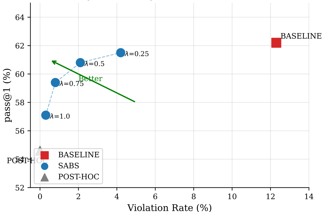
Quality vs. Security Trade-off on HumanEval
