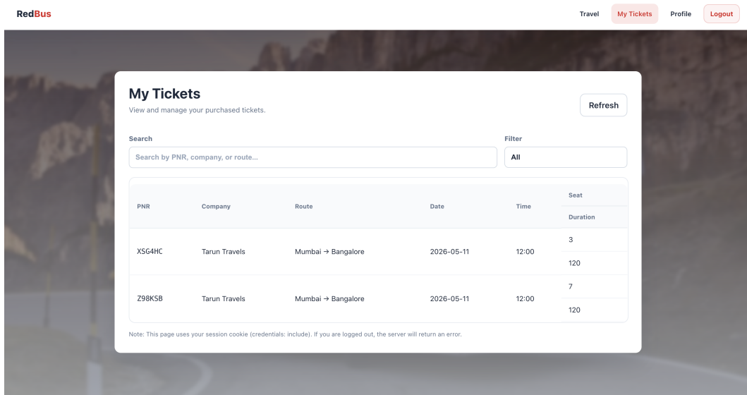
Figure 6: Additional frontend state in role-aware navigation
