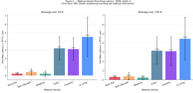
Fig. 3. Ping-Pong Latency Across All Six SHM Wakeup Variants. Spinning variants achieve sub-microsecond latency at small sizes; kernel-sleeping variants converge to 3–5 \mu s. All six converge near 150–155 \mu s at 1 MiB, confirming memory bandwidth as the common bottleneck.
