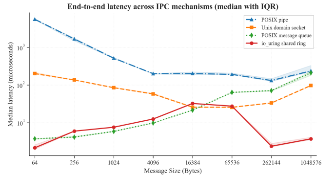
Fig. 7. Median (P50) Latency ( \mu\text{s} , log scale) vs. Message Size under saturated load. These are queued-latency measurements (not corrected unloaded latency). POSIX Pipe reaches 5,102\ \mu\text{s} at 64 B due to accumulated queuing and context-switch overhead.
