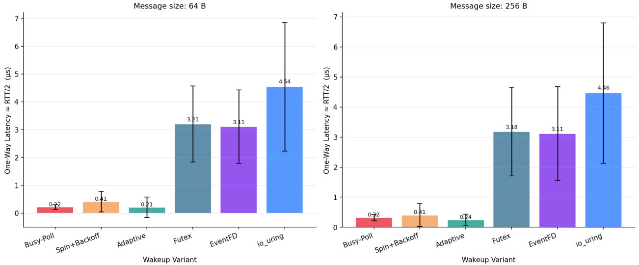
Fig. 3. Ping-Pong Latency Across All Six SHM Wakeup Variants. Spinning variants achieve sub-microsecond latency at small sizes; kernel-sleeping variants converge to 3\text{--}5\ \mu\text{s} . All six converge near 150\text{--}155\ \mu\text{s} at 1 MiB, confirming memory bandwidth as the common bottleneck.
