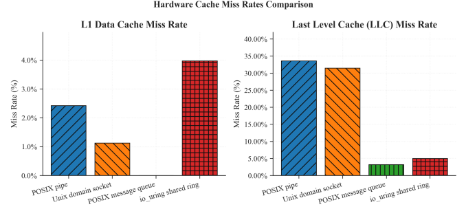
Fig. 9. L1 D-Cache and LLC Miss Rates by IPC Mechanism. Pipe and Socket exhibit \approx 30–34 % LLC miss rates due to kernel buffer staging evicting ring cache lines. SHM Ring (4.97 %) and POSIX MQ (3.2 %) achieve low LLC miss rates by keeping data in the shared 18 MiB L3.
