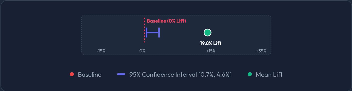
Interval Chart: Relative Lift Estimate (Confidence Interval)
