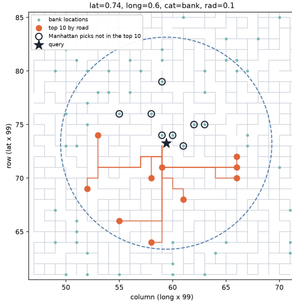
Figure 1: Query lat=0.74, long=0.6, cat=bank, rad=0.1. Grey lines are links (gaps are missing links); orange shows the 10 results and the paths to them; circled points are what Manhattan ranking would return instead.
