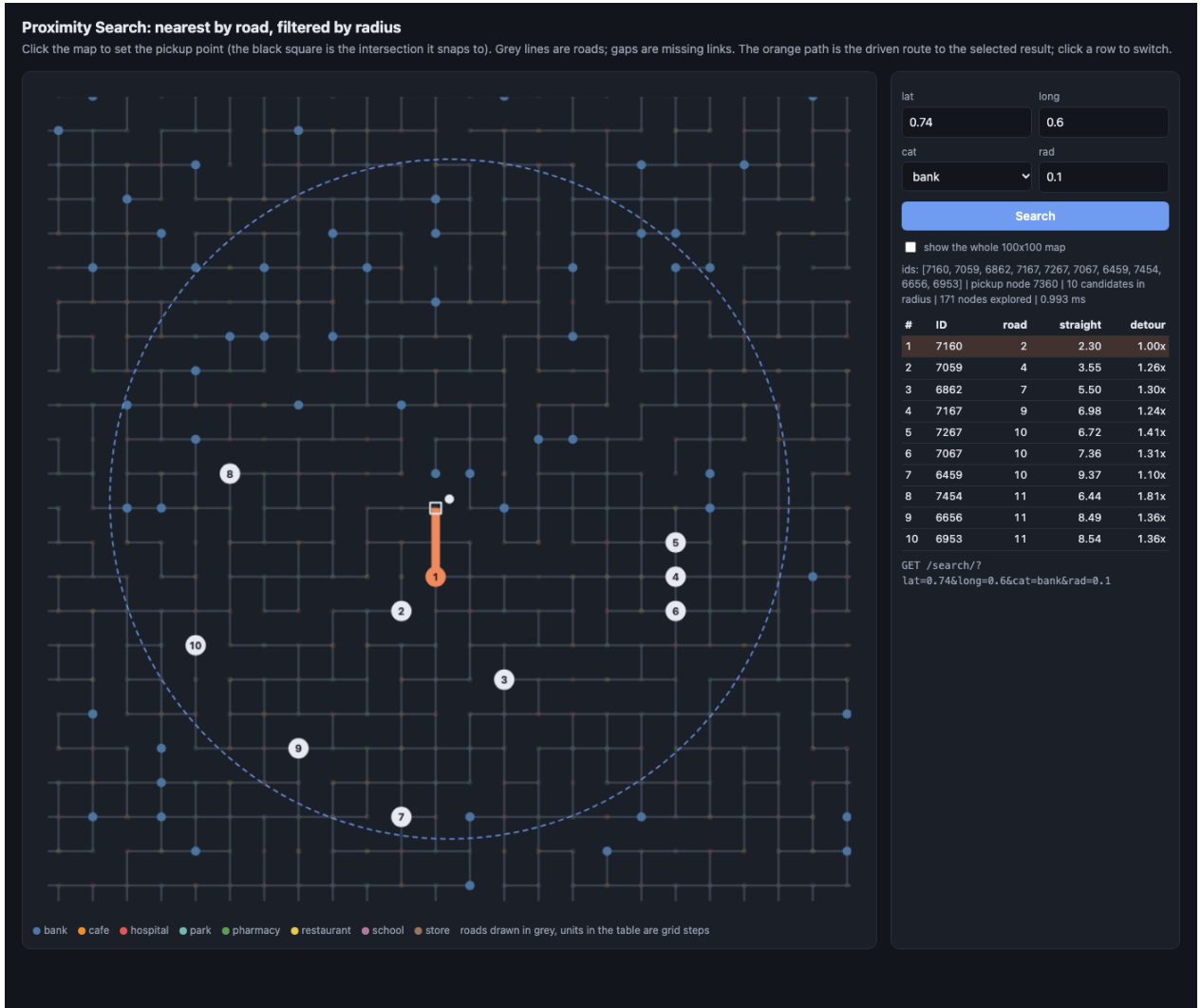
Figure 2: The deployed API answering the example query. The square is the grid point the query snaps to, and the orange line is the path to result 1.
