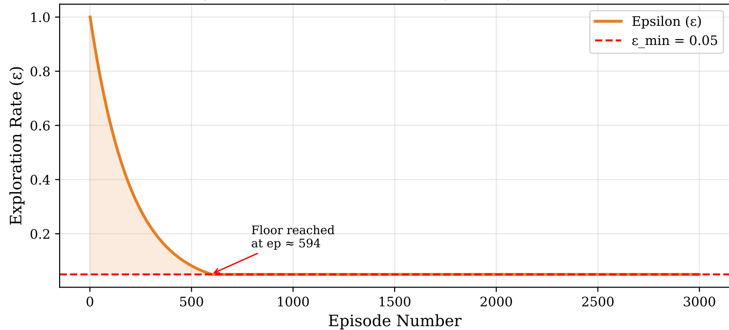
Figure 4.2 — Epsilon-Greedy Decay Schedule
