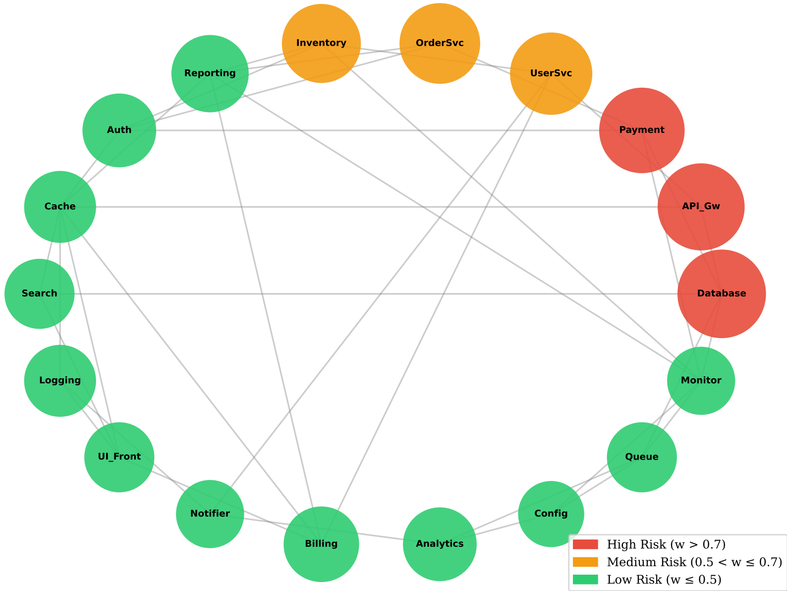
Figure 2.1 — Software Module Graph (Watts-Strogatz, 18 nodes)
