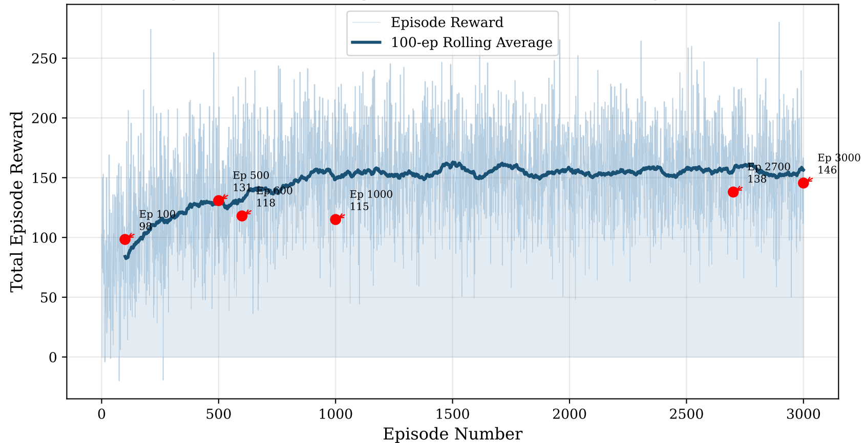
Figure 4.1 — Learning Curve: Reward over Training Episodes
