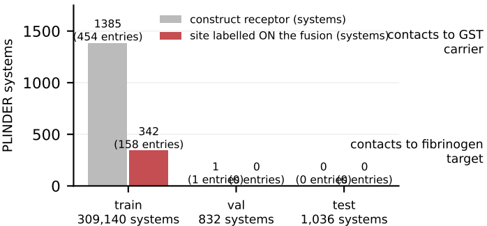
B PLINDER 2024-06/v2, by split (system and unique-entry counts both shown)
