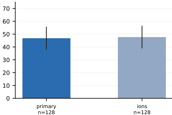
fpocket
