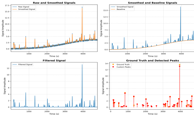
Figure: Raw, smoothed, baseline, and filtered signals processed using the custom method, along with detected peaks and ground truth peaks for comparison.
