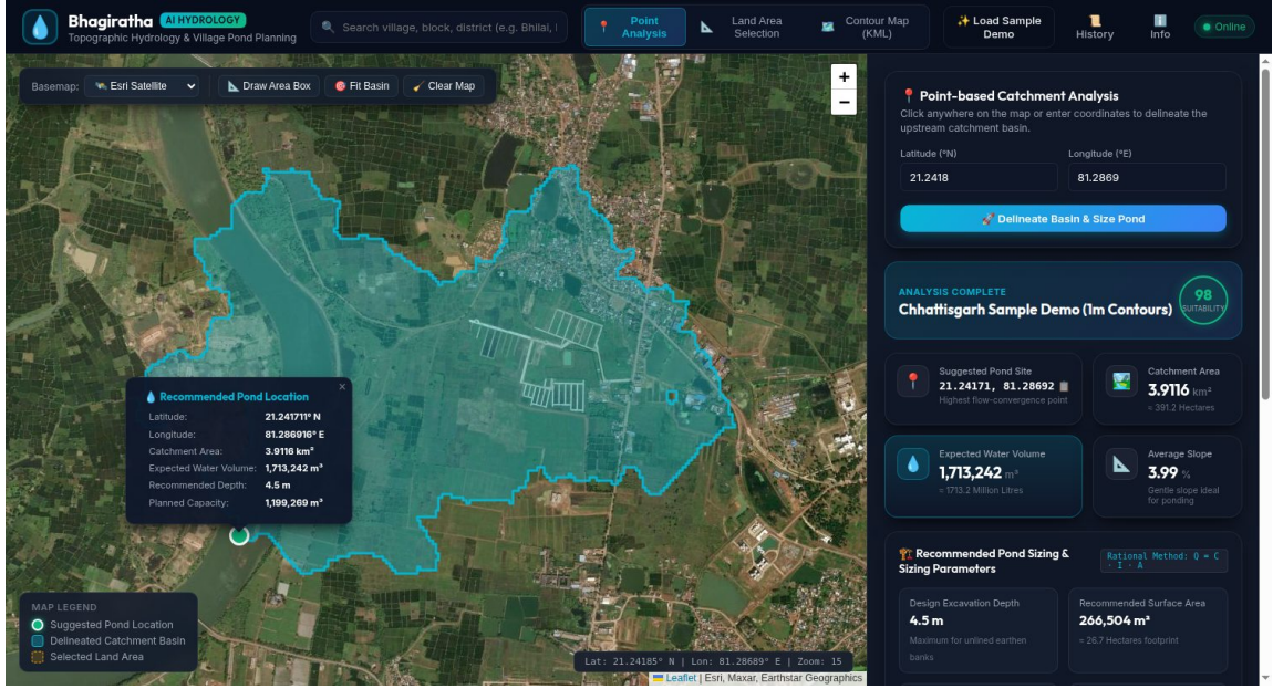
Fig. 2. Application interface after the sample contour analysis: catchment polygon, pond marker with its popup (location, catchment area, expected water volume, depth, capacity) and the results panel.
