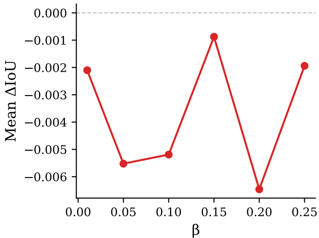
Mean \Delta\text{IoU} vs \beta
