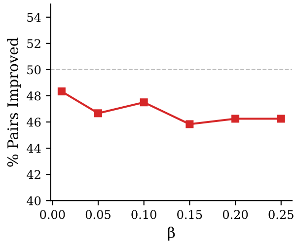
Improvement Rate vs \beta
