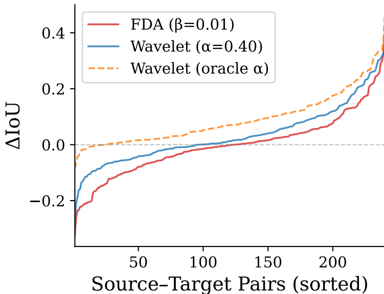
Oracle \alpha vs Fixed \alpha
