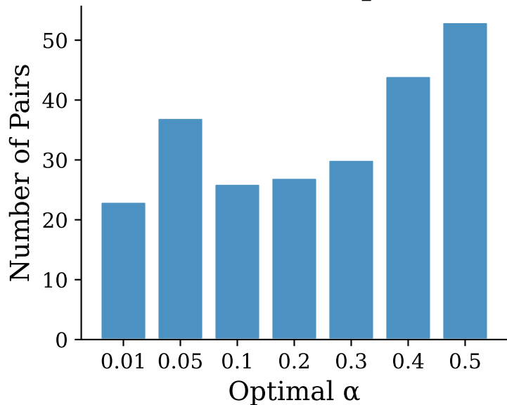
Distribution of Optimal \alpha
