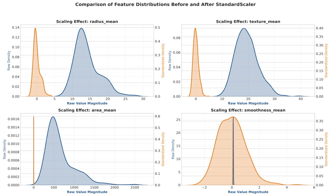
Figure 2: Distribution Densities Before vs. After Feature Standardization (StandardScaler)
