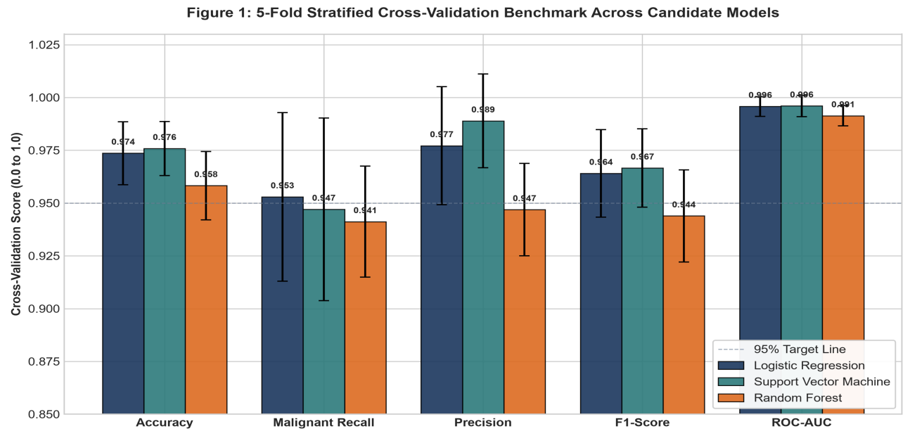
Figure 1: 5-Fold Stratified Cross-Validation Benchmark Across Candidate Models
