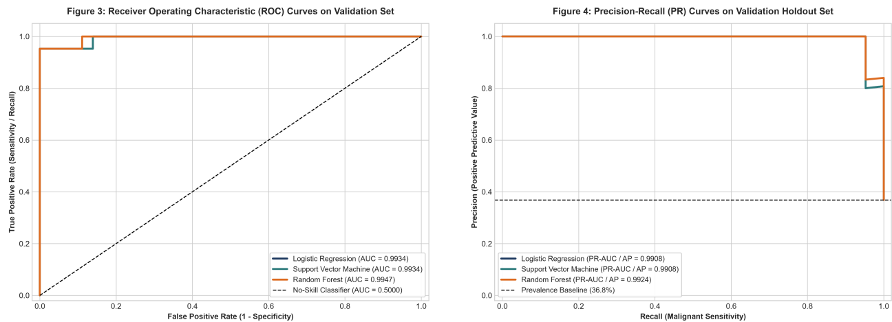
Figure 3: Discrimination Diagnostics: Validation ROC Curves vs. Precision-Recall Curves
