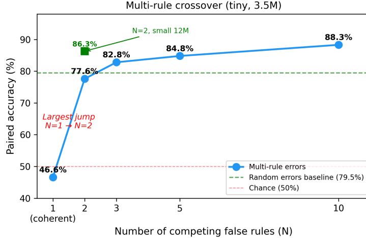
Figure 2: Multi-rule crossover. Accuracy jumps from 47% ( N=1 ) to 78% ( N=2 ), then grows gradually through N=10 . X-axis is categorical (not log-scale); point spacing does not represent proportional distances.
