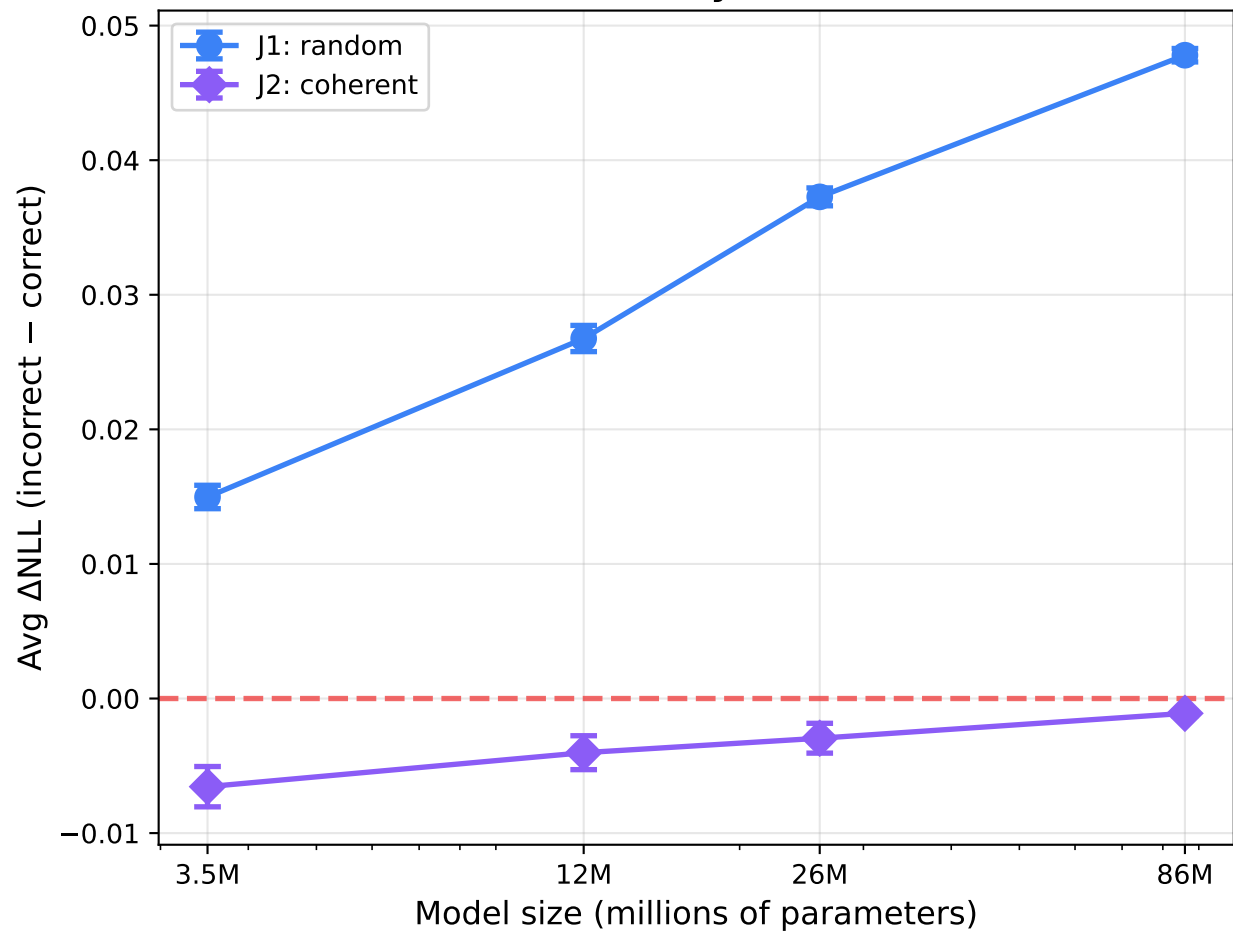
Paired \Delta NLL by Model Size
