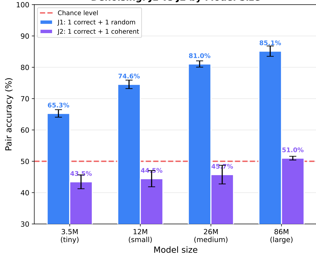
Denoising: J1 vs J2 by Model Size
