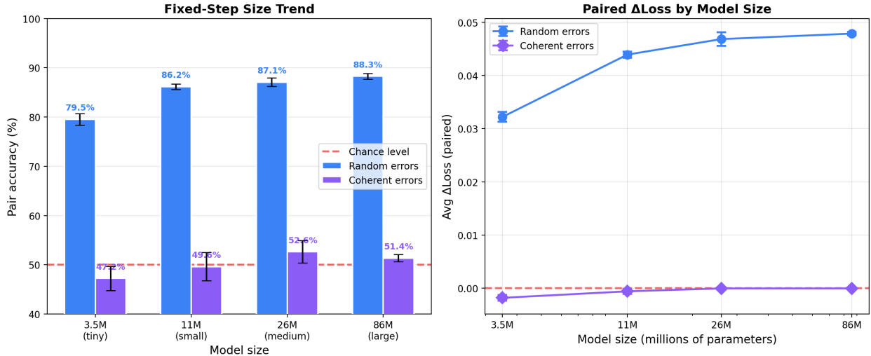
Figure C1. Scaling in the standard setup. Random accuracy rises from 80% to 88%; coherent accuracy stays near chance (47–53%) across the 3.5M–86M range.
