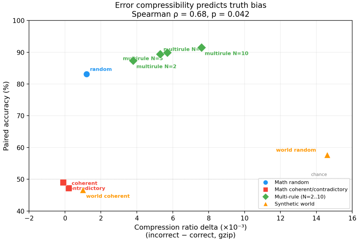
Figure B1. Compression ratio delta (gzip, incorrect minus correct) vs paired accuracy. Spearman \rho = 0.68 , p = 0.042 . Coherent and contradictory errors cluster near zero delta and chance accuracy; random and multi-rule errors show progressively larger deltas.
