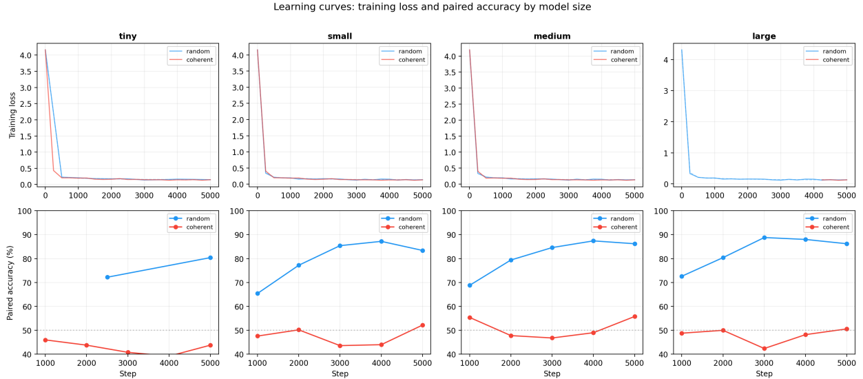
Figure E2. Learning curves. All sizes reach behavioral plateau by step 3000–4000. The large model achieves 88.8% at step 3000, stable through 5000. Coherent models stay near chance throughout.
