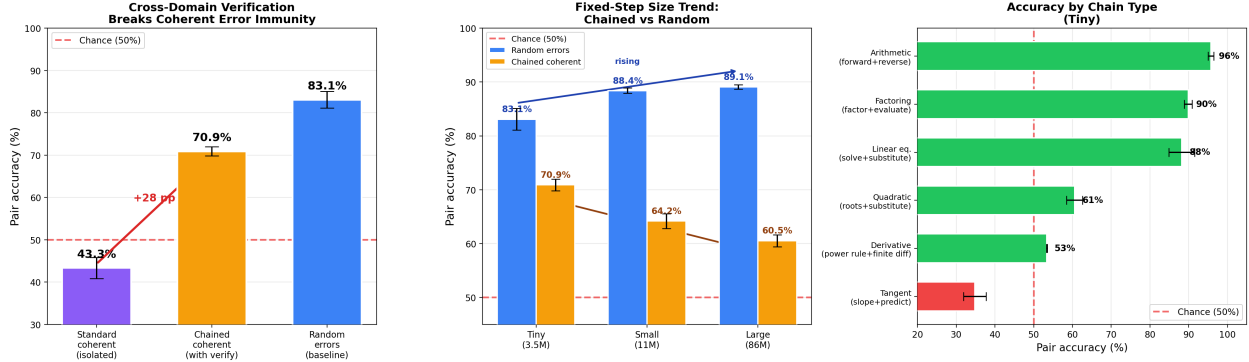
Figure E1. Chained verification restores truth bias from 43% to 71% at tiny, but the effect weakens at larger model sizes. Control: truncated chains without verification yield 44.3% – same as standard coherent.
