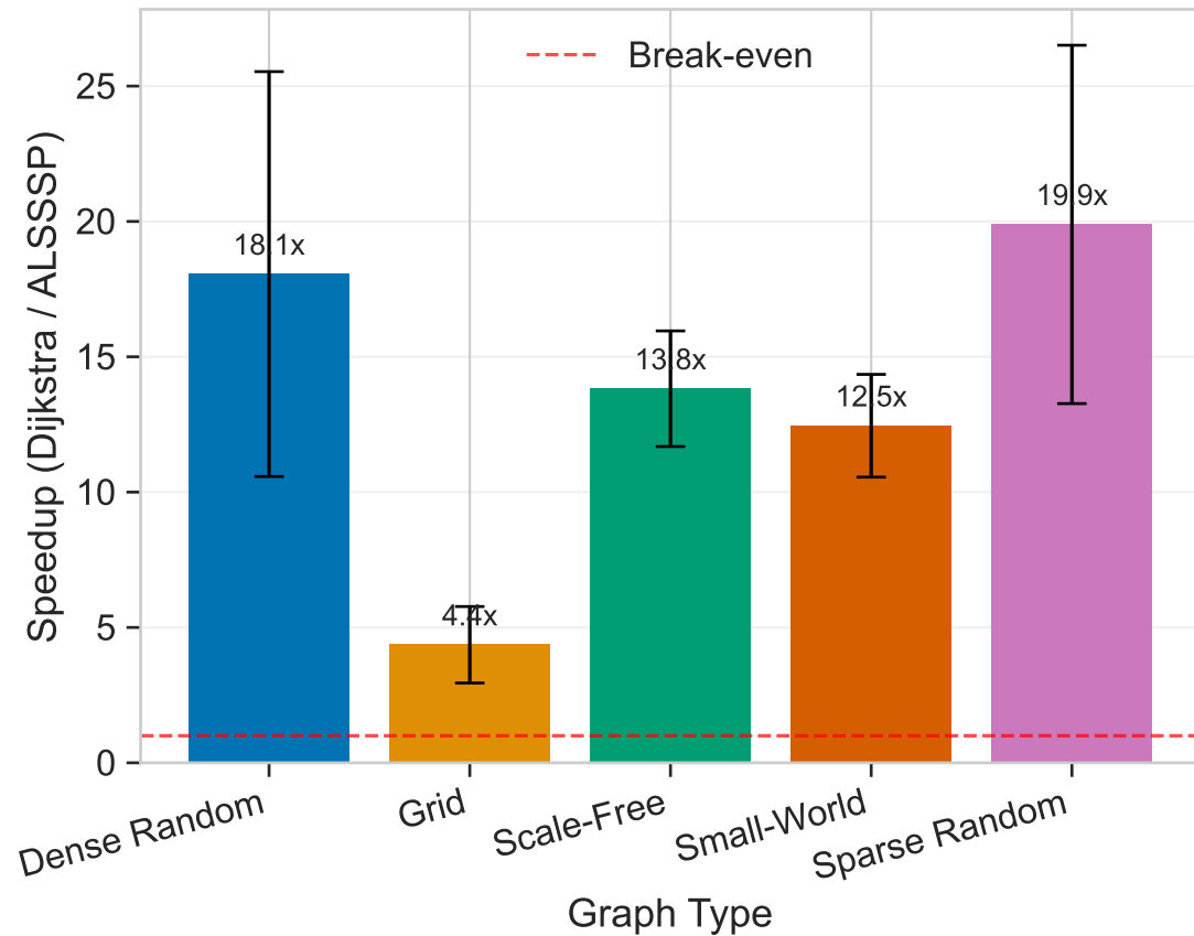
(b) ALSSSP Speedup by Graph Type
