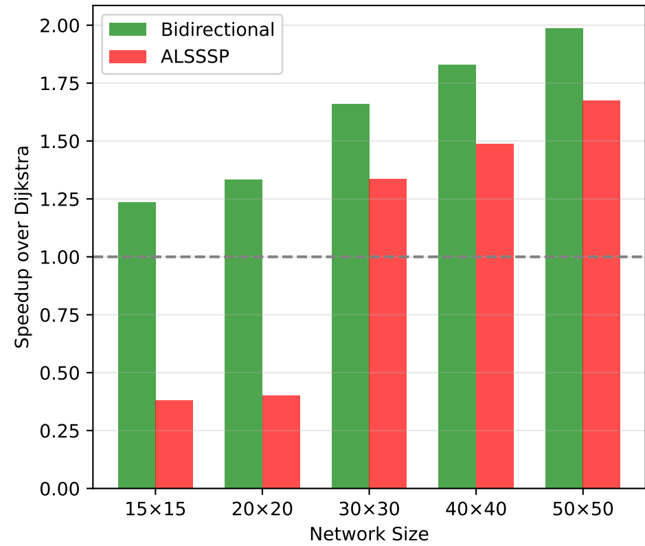
Speedup Factor
