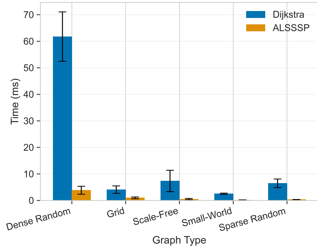
(a) Point-to-Point Query Time by Graph Type
