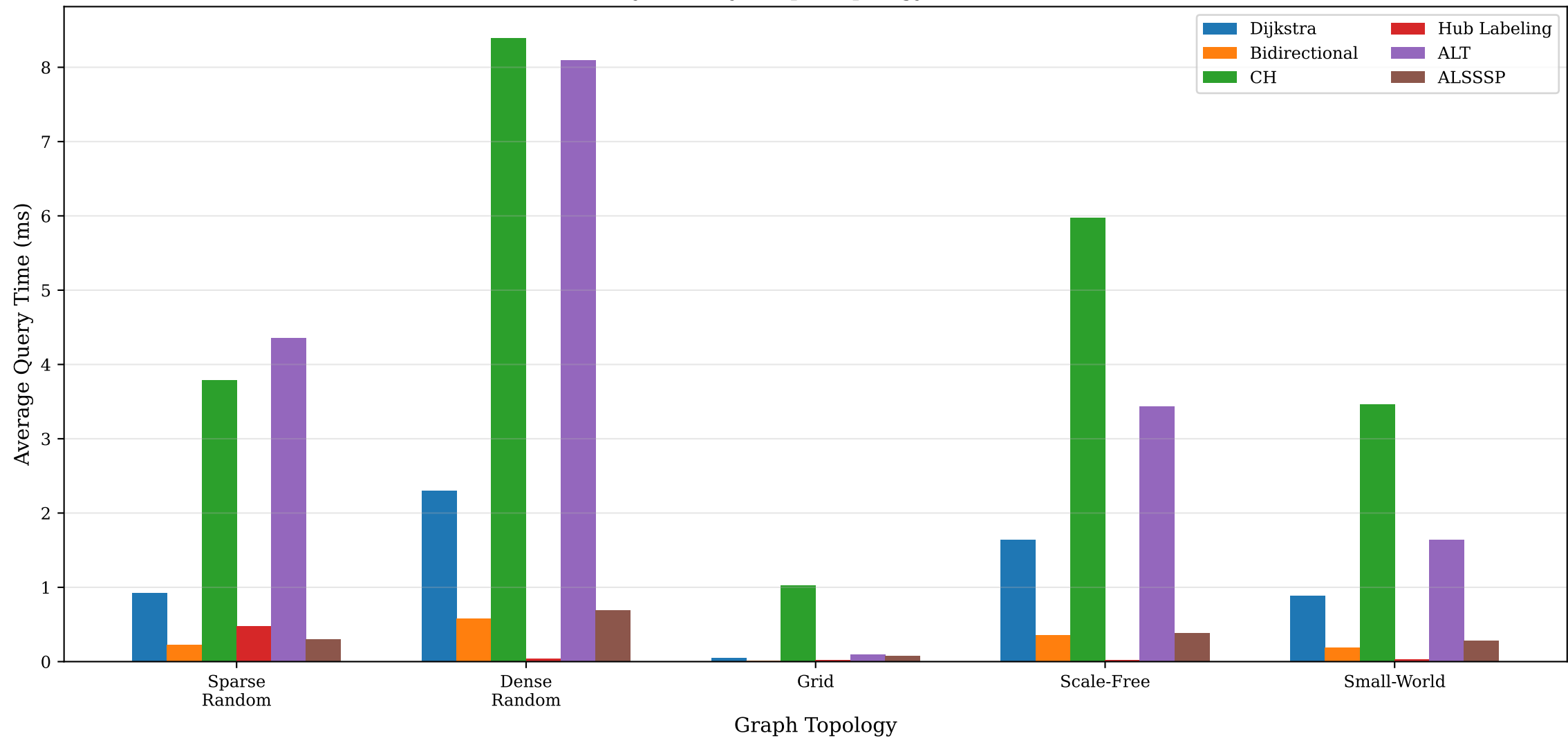
Query Time by Graph Topology (n ≈ 2000)
