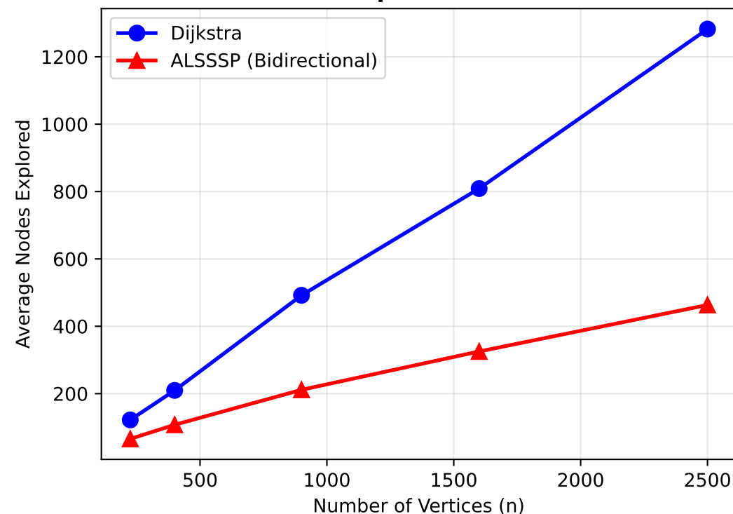
Search Space Reduction
