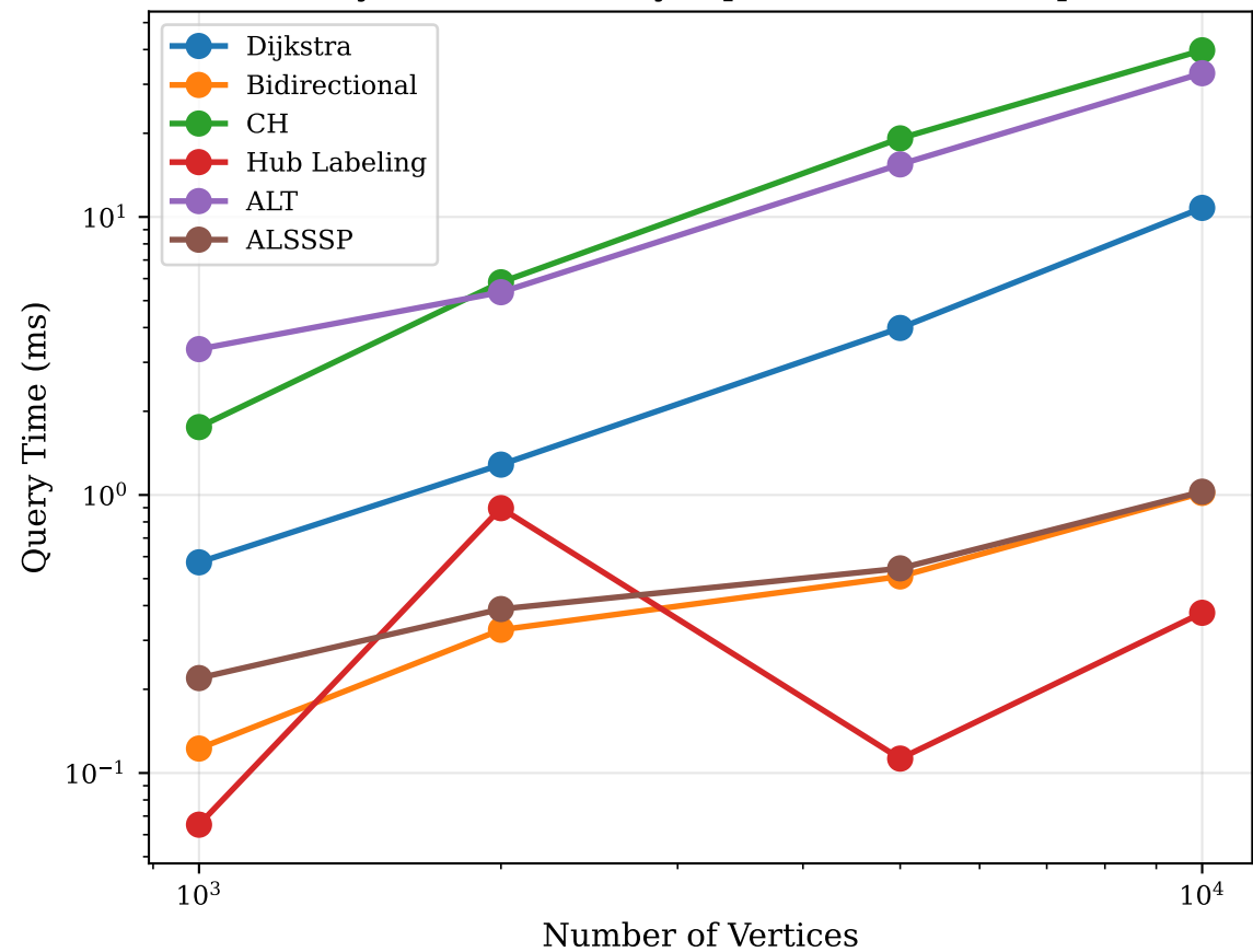
Query Time Scalability (Sparse Random Graphs)
