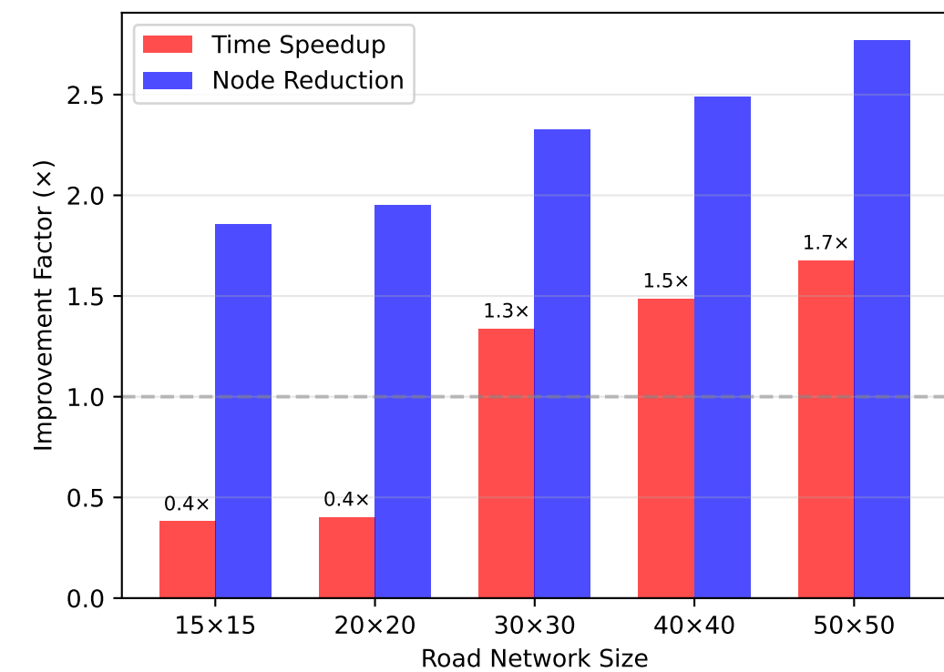
ALSSSP Performance Gains
