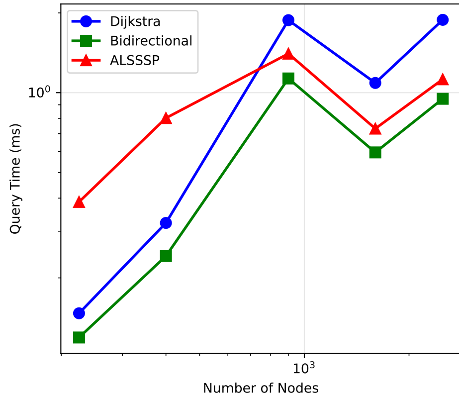
Query Time on Road Networks
