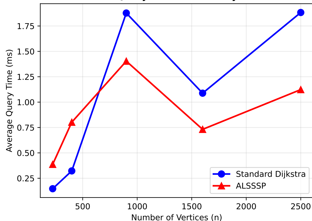
Query Time Scalability
