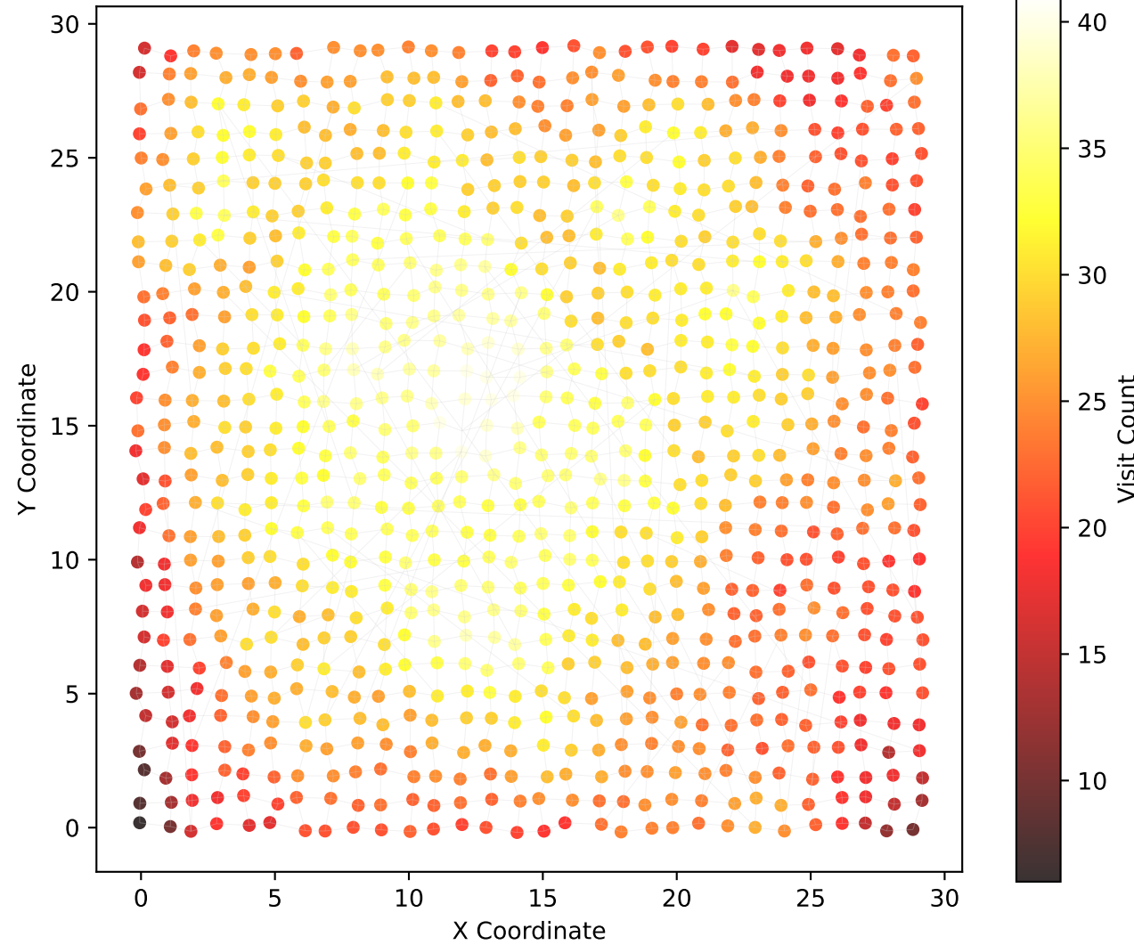
Dijkstra Exploration Frequency (Total visits: 24597)
