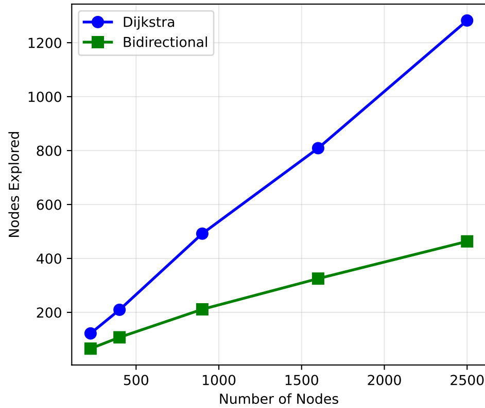
Exploration Efficiency
