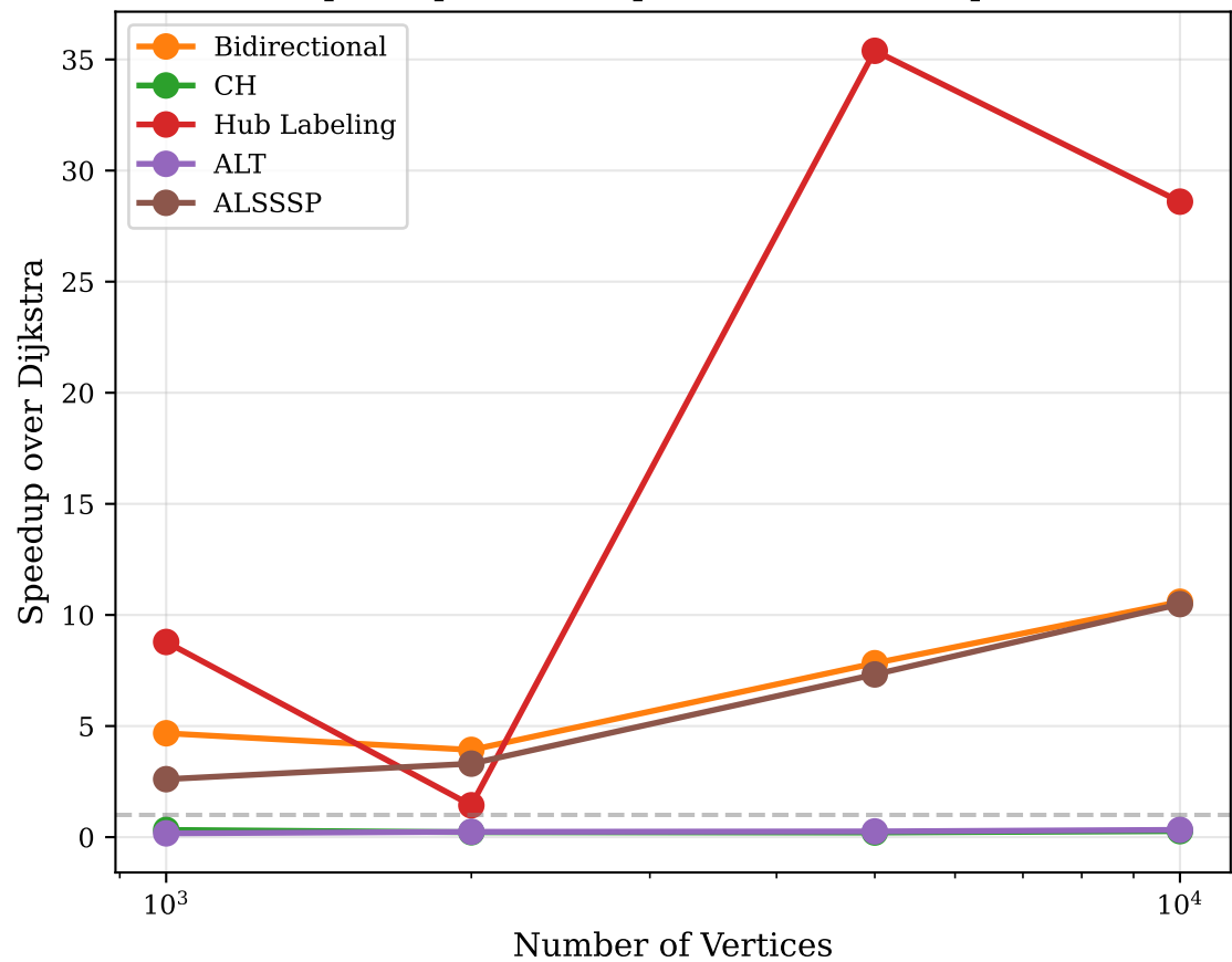
Speedup Factor (Sparse Random Graphs)
