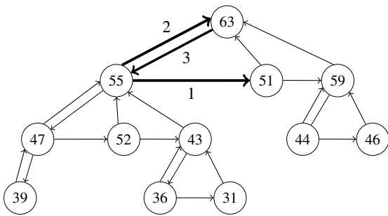
Melding Pairing Heaps Using Parent Pointers
