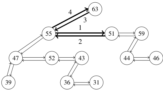
Melding Pairing Heaps Using Previous Pointers
