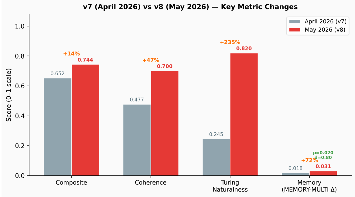
Figure 2: Key metric improvements from April 2026 (v7, 217 cocoons) to May 2026 (v8, 951 cocoons). Turing naturalness improves by 235% (0.245 \rightarrow 0.820), resolving the depth–naturalness tradeoff documented in v7. Memory augmentation delta increases from 0.018 to 0.031 and reaches statistical significance ( p = 0.020 , d = 0.80 ).
