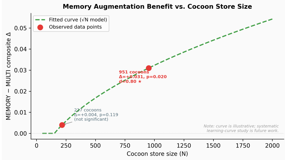
Figure 5: Memory augmentation benefit ( \Delta composite, MEMORY – MULTI) vs. cocoon store size. Two observed data points: non-significant at 217 cocoons ( \Delta = +0.004 , p = 0.119 ); large-effect significant at 951 cocoons ( \Delta = +0.031 , p = 0.020 , d = 0.80 ). Curve is a \sqrt{N} fit for illustration; systematic study is future work.
