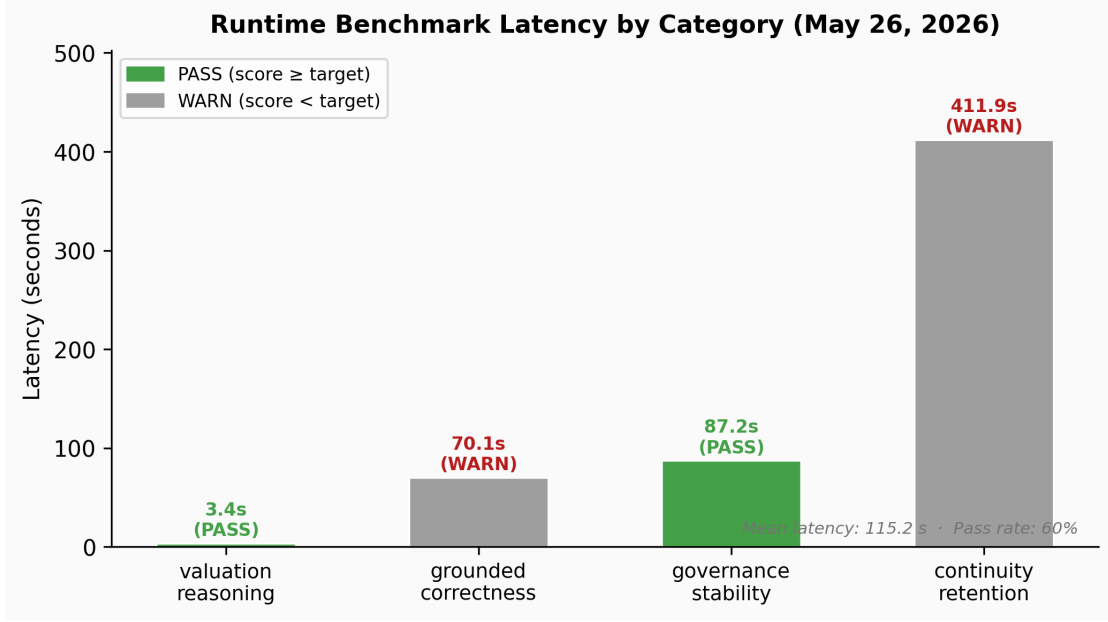
Figure 4: Runtime benchmark latency by category (May 26, 2026). Green bars indicate passing cases (score \geq target); grey bars indicate warnings. Valuation-reasoning queries (pre-computed graph traversal) complete in \sim 3.4 s; continuity-retention requires multi-turn context loading ( \sim 412 s). Mean latency: 115.2 s; pass rate: 60%.
