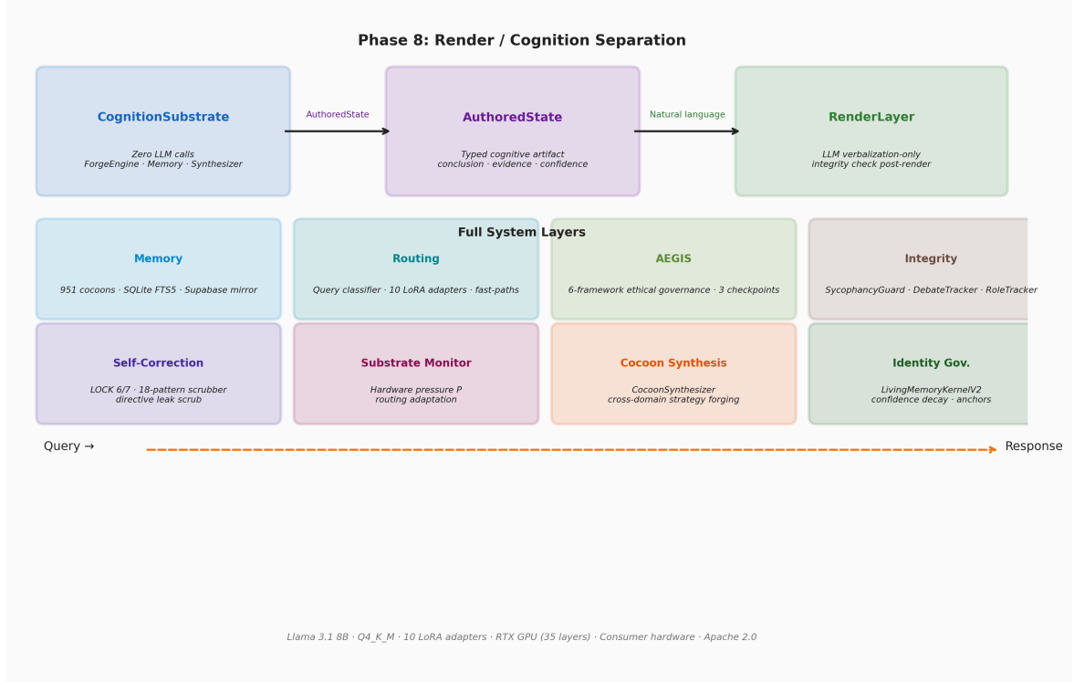
Figure 1: CODETTE v8 layered architecture. The top row shows the Phase 8 render/cognition pipeline (section 5): COGNITIONSUBSTRATE (zero LLM calls) produces an AUTHOREDSTATE, which RENDERLAYER expresses in natural language. The lower rows show the full system layers through which every query passes.
