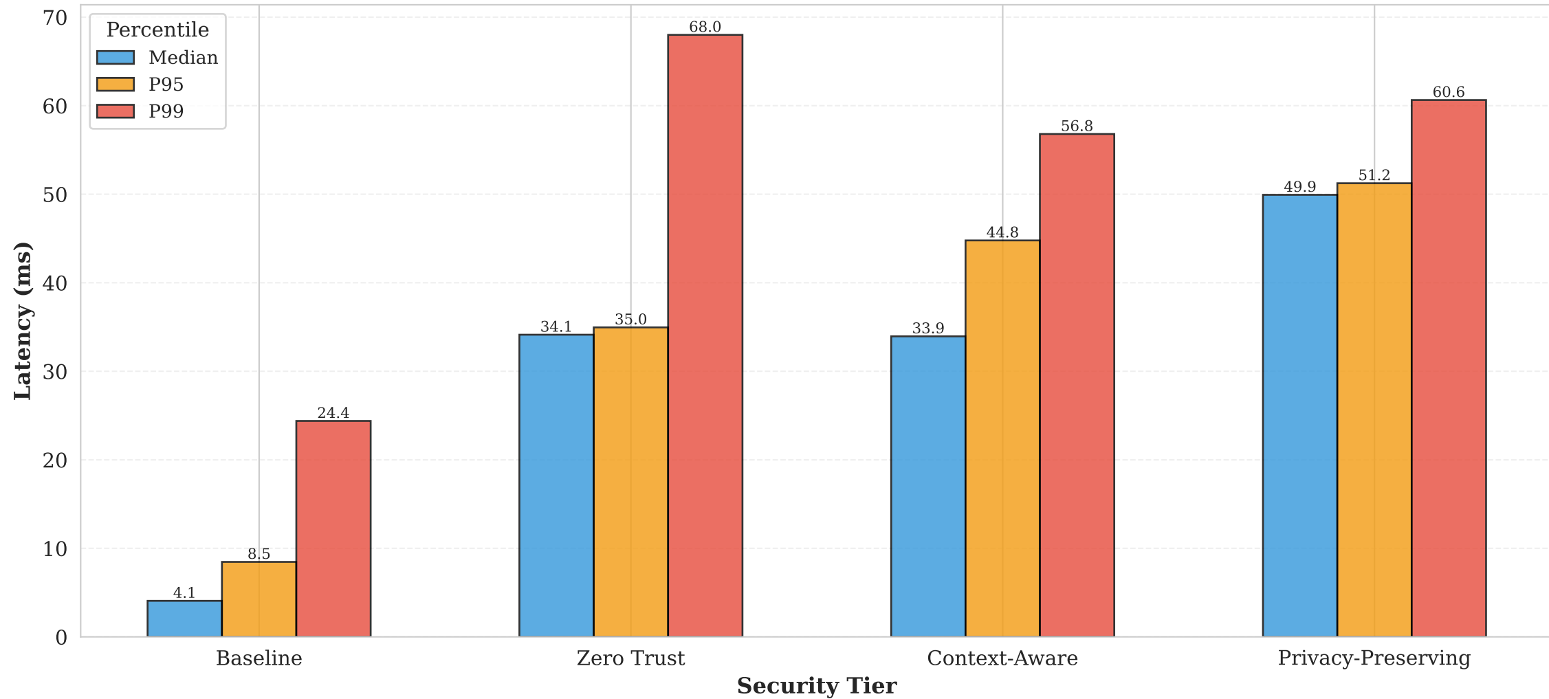
Latency Distribution Across Security Tiers
