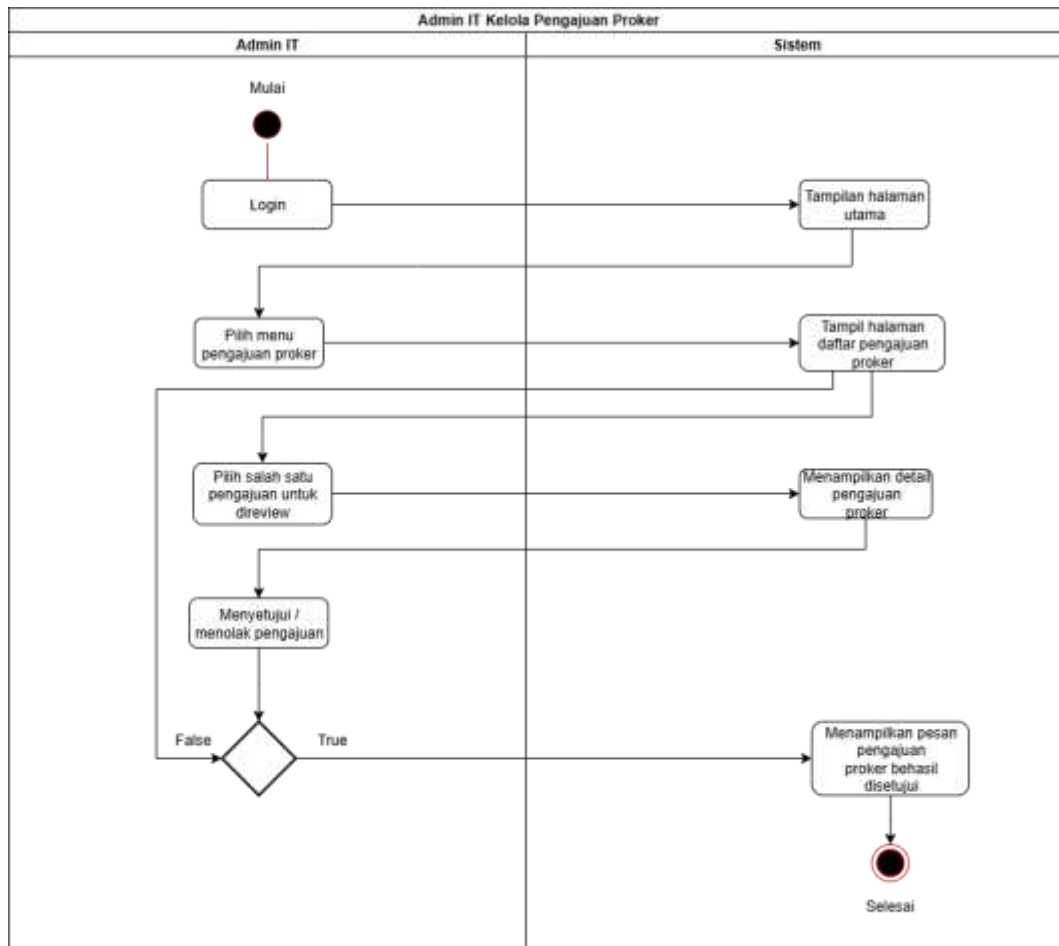
Gambar 4.8 Activity Diagram Admin IT Kelola Pengajuan Proker
