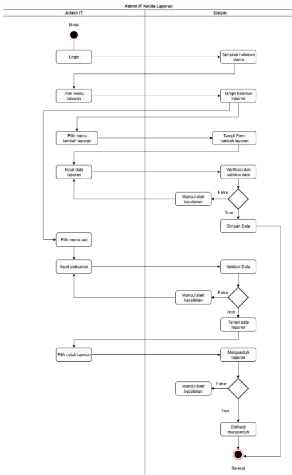
Gambar 4.10 Activity Diagram Admin IT Kelola Laporan
