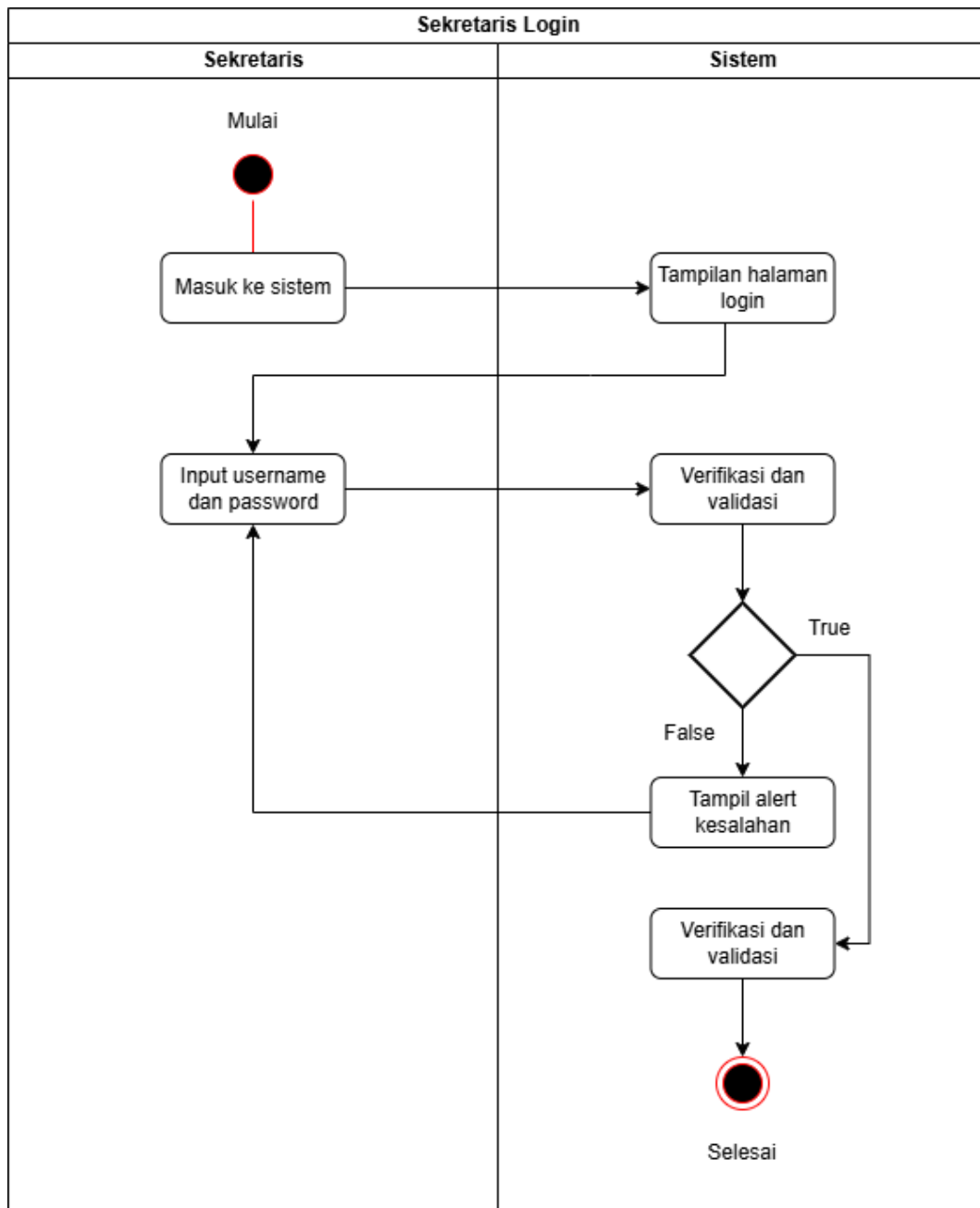
Gambar 4.19 Activity Diagram Sekretaris Login
