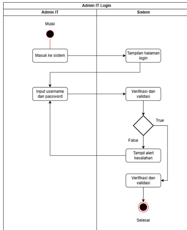
Gambar 4.3 Activity Diagram Admin IT Login
