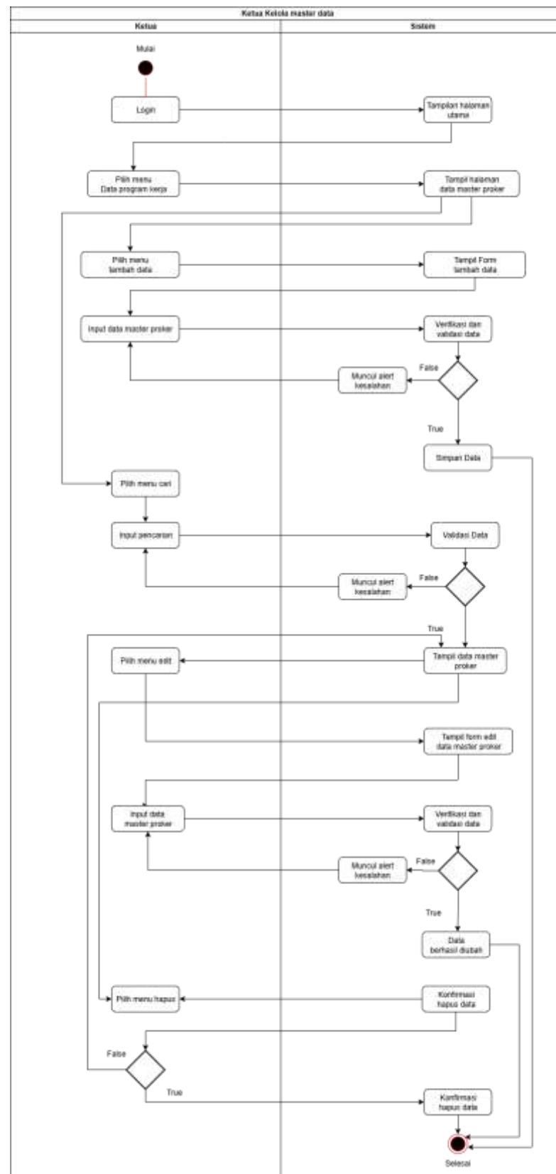
Gambar 4.15 Activity Diagram Ketua Kelola Master Data Program Kerja
