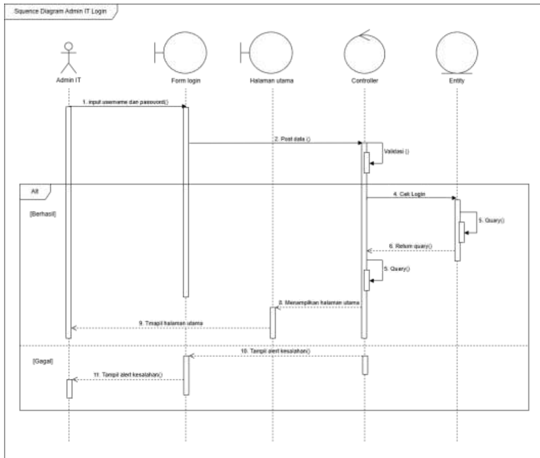
Gambar 4.27 Sequence Diagram Admin IT Login
