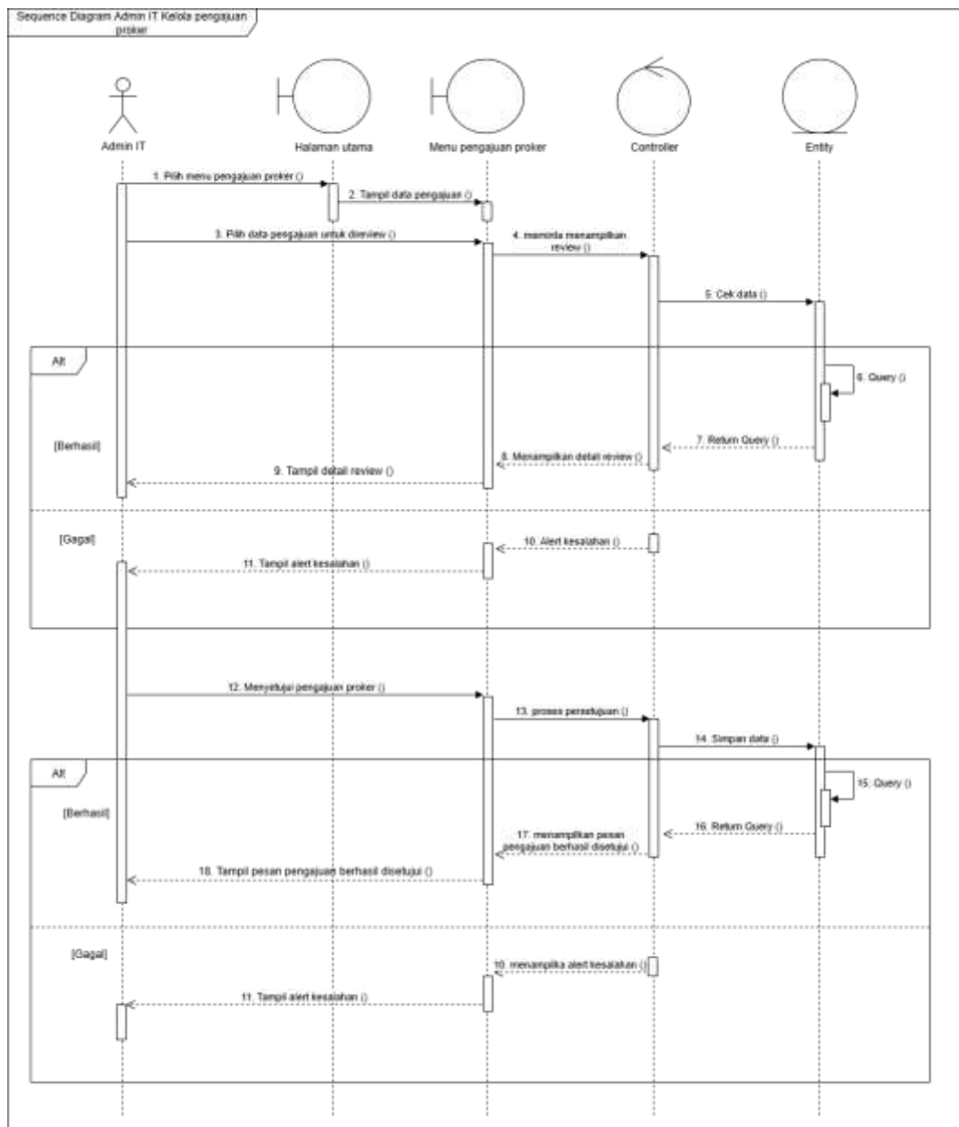
Gambar 4.32 Sequence Diagram Admin IT Kelola Pengajuan Program Kerja
