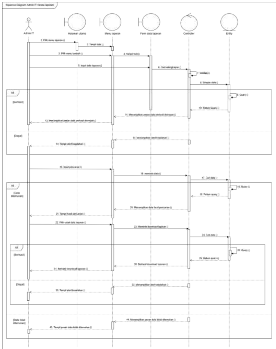
Gambar 4.34 Sequence Diagram Admin IT Kelola Laporan
