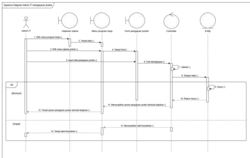
Gambar 4.30 Sequence Diagram Admin IT Mengajukan Program Kerja
