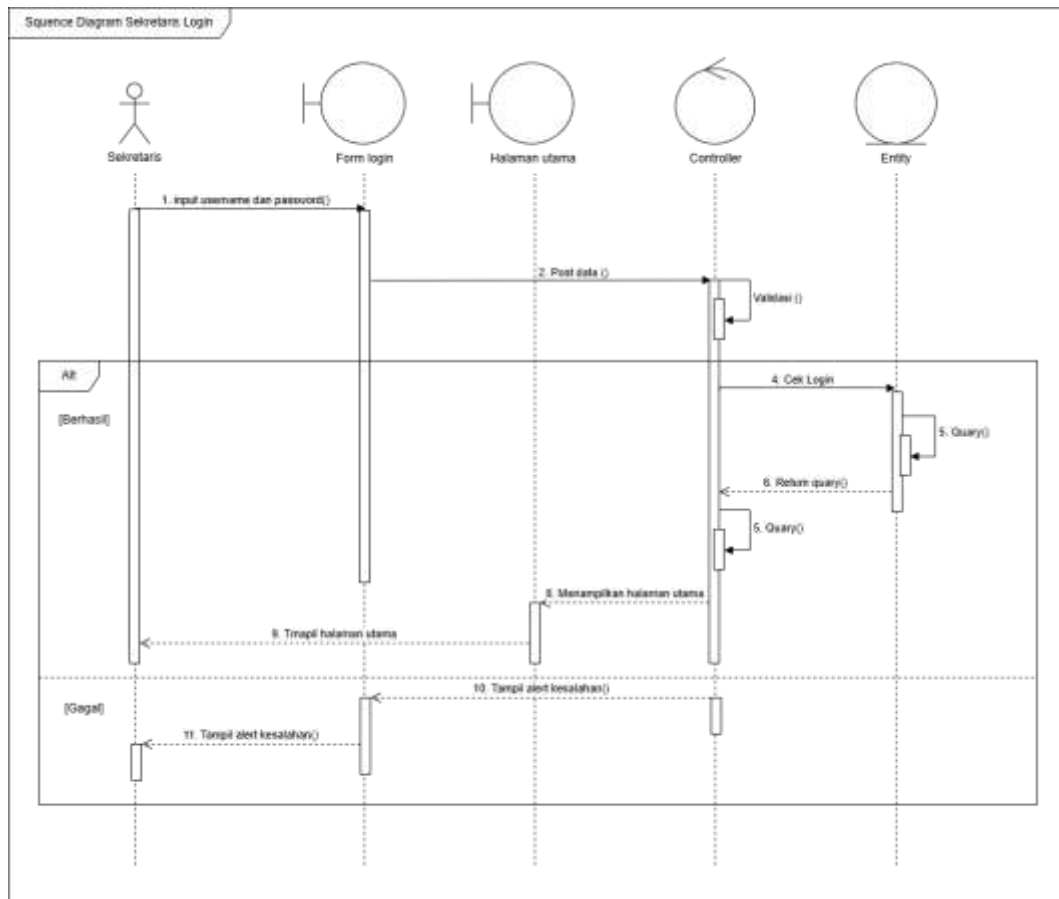
Gambar 4.43 Sequence Diagram Sekretaris Login
