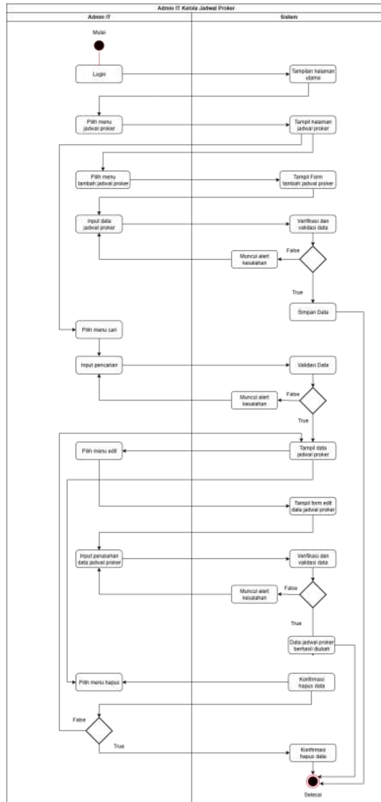
Gambar 4.9 Activity Diagram Admin IT Kelola Jadwal Proker
