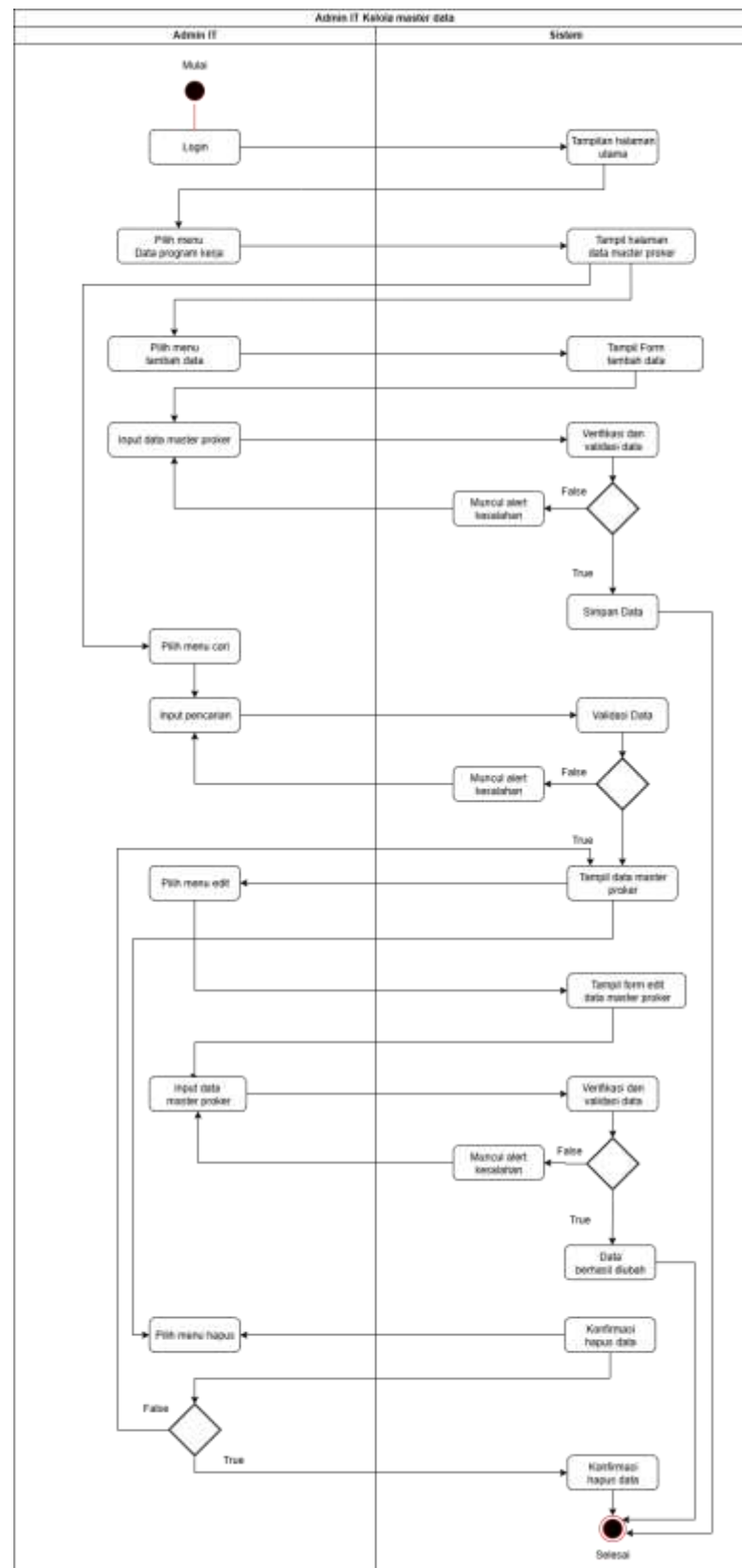
Gambar 4.7 Activity Diagram Admin IT Kelola Master Data Program Kerja
