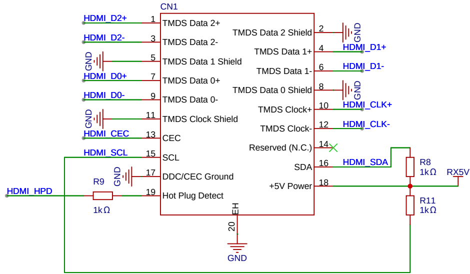
HDMI IN
