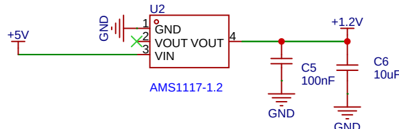
5V-1.2V LDO
