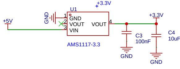
5V-3.3V LDO
