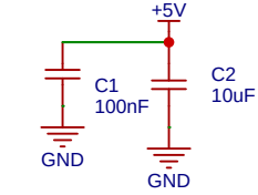
POWER IN
